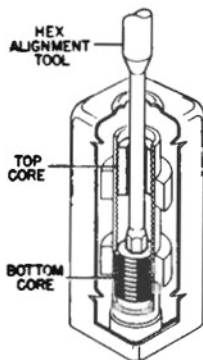
IF ALIGNMENT DETAIL
