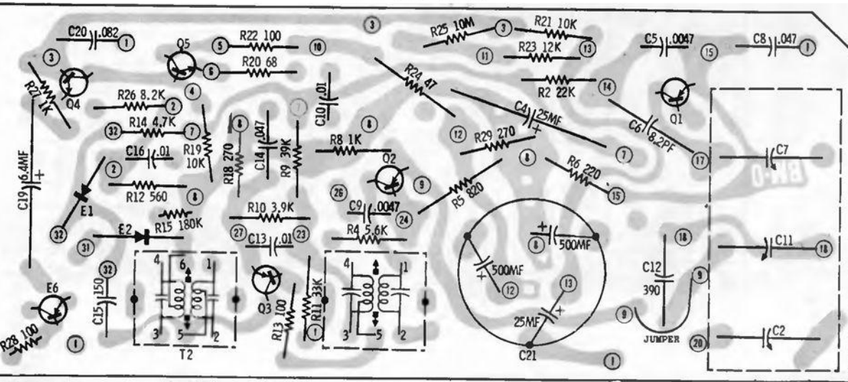
BOTTOM VIEW
