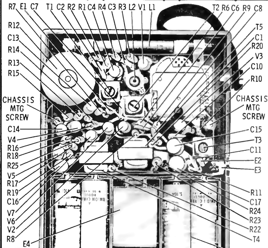
MODEL X38 PARTS LOCATION
