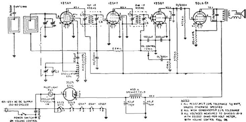
CIRCUIT DIAGRAM
