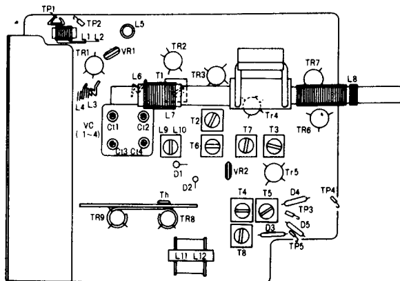
LOCATION OF PART (FOR ALIGNMENT)
