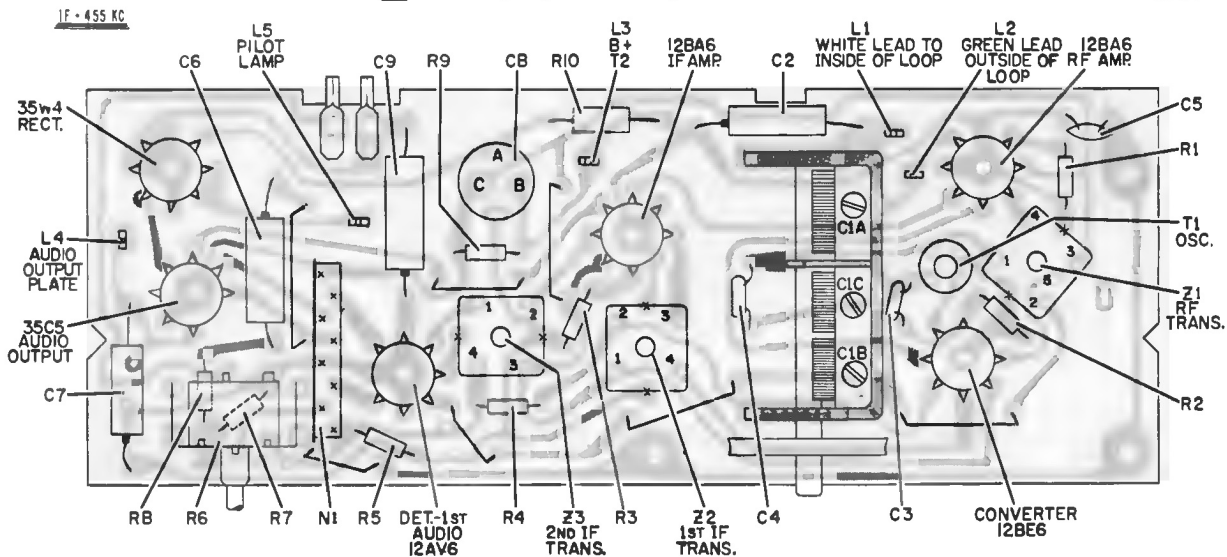
Composite View, Component Layout of Printed Panel
