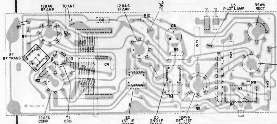
Composite Bottom View, Perma-Circuit Panel
