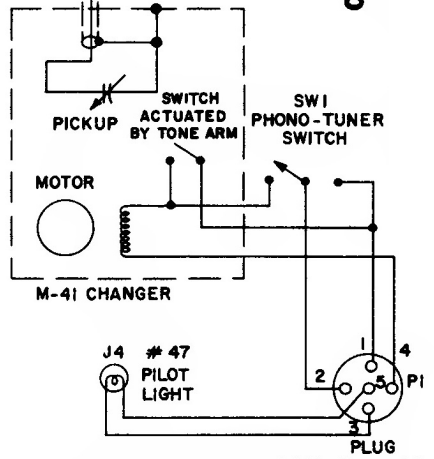
Additional Circuitry for Model G-1606
