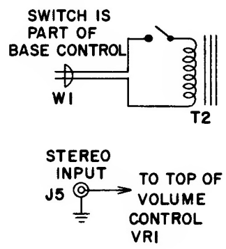
Additional Circuitry for Model SA-1000
