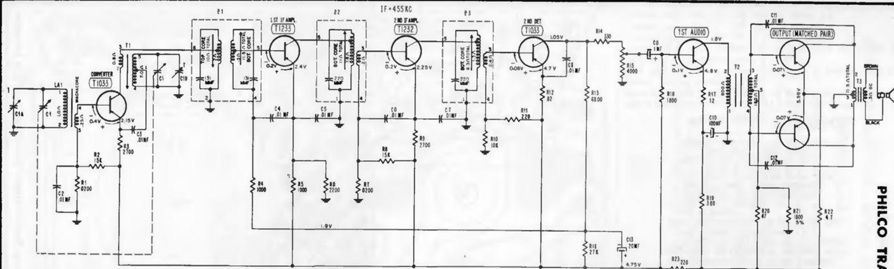
Schematic Diagram of Model T-78
