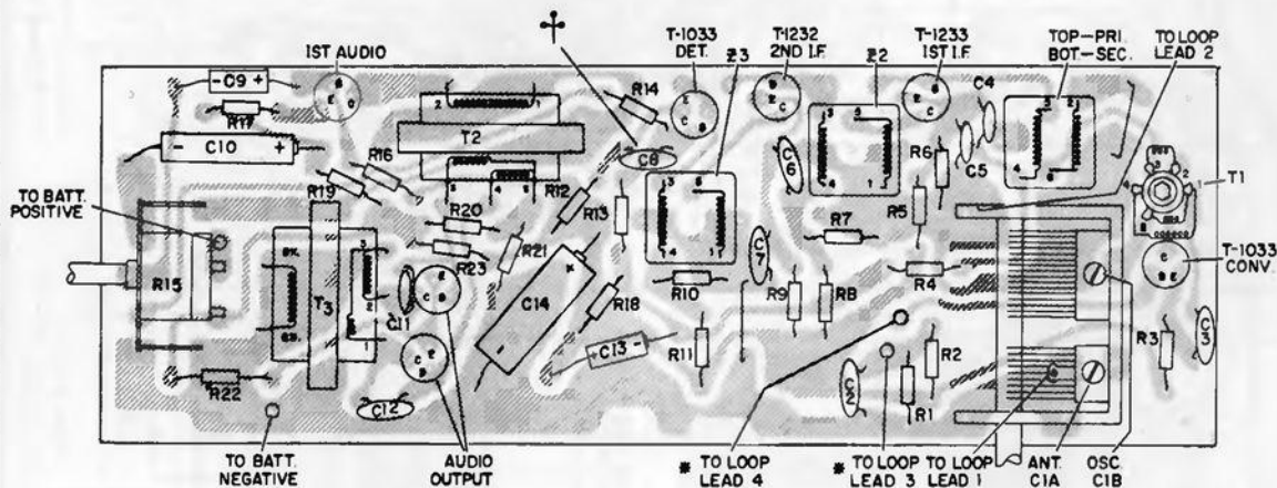
Top View, PW Panel
