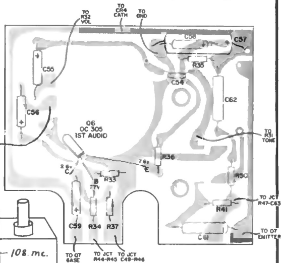
Bottom View Audio Driver Stage
