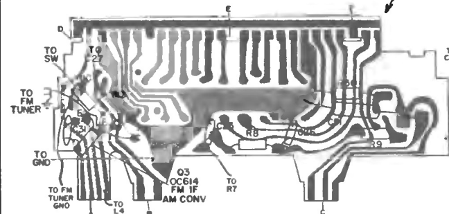
Top View - Pushbutton Assy. Top-
