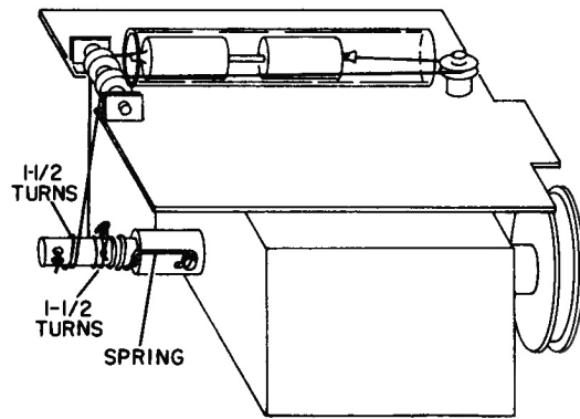
FM Tuner Dial Cord
