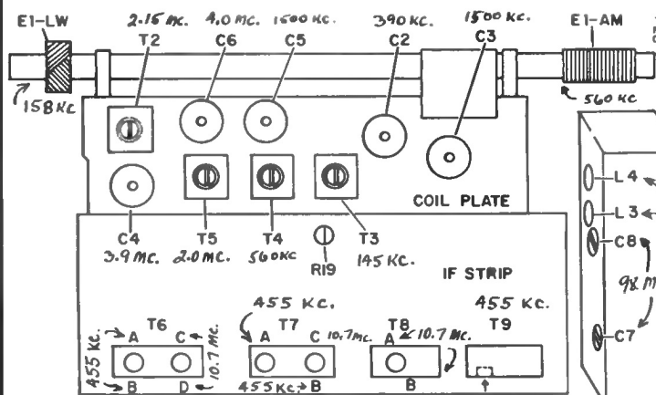
Alignment Points for AM, FM, LW & SW
