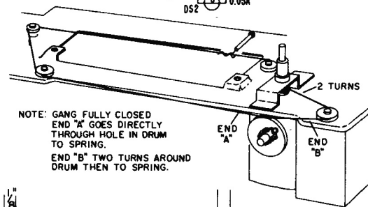
Dial Cord Stringing
