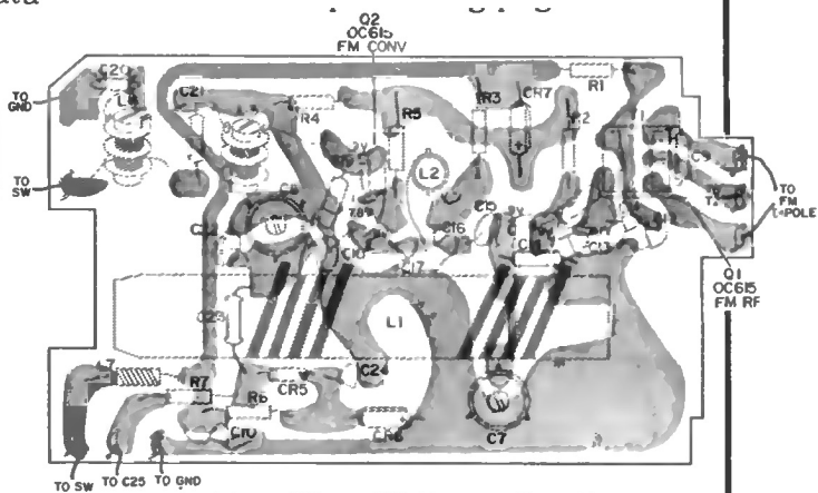
Bottom View FM Tuner Panel
