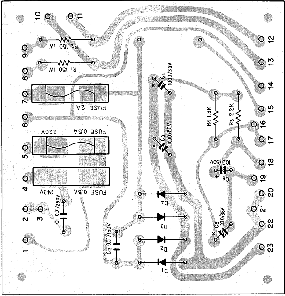
Power supply ass'y KWR-801
