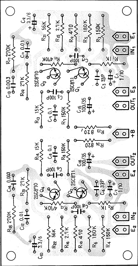
Equalizer amp ass'y AWF-001
