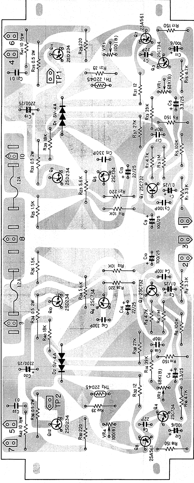
Power amp ass'y AWH-005
