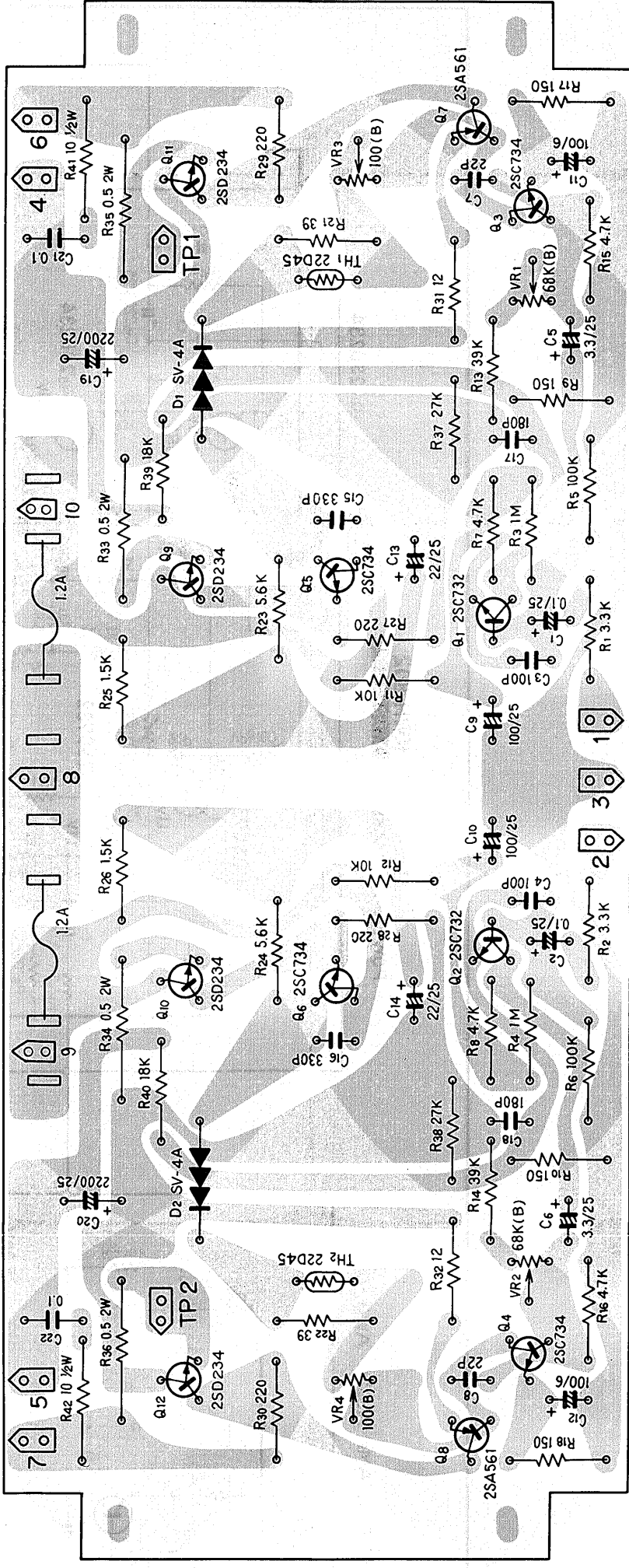
Power amp ass'y KWH-802
