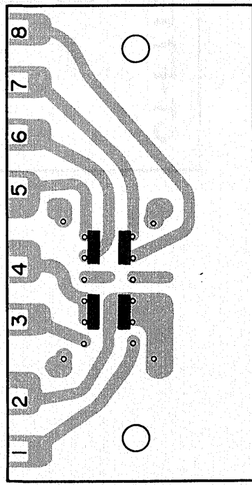
Switch circuit ass'y C RWS-010
