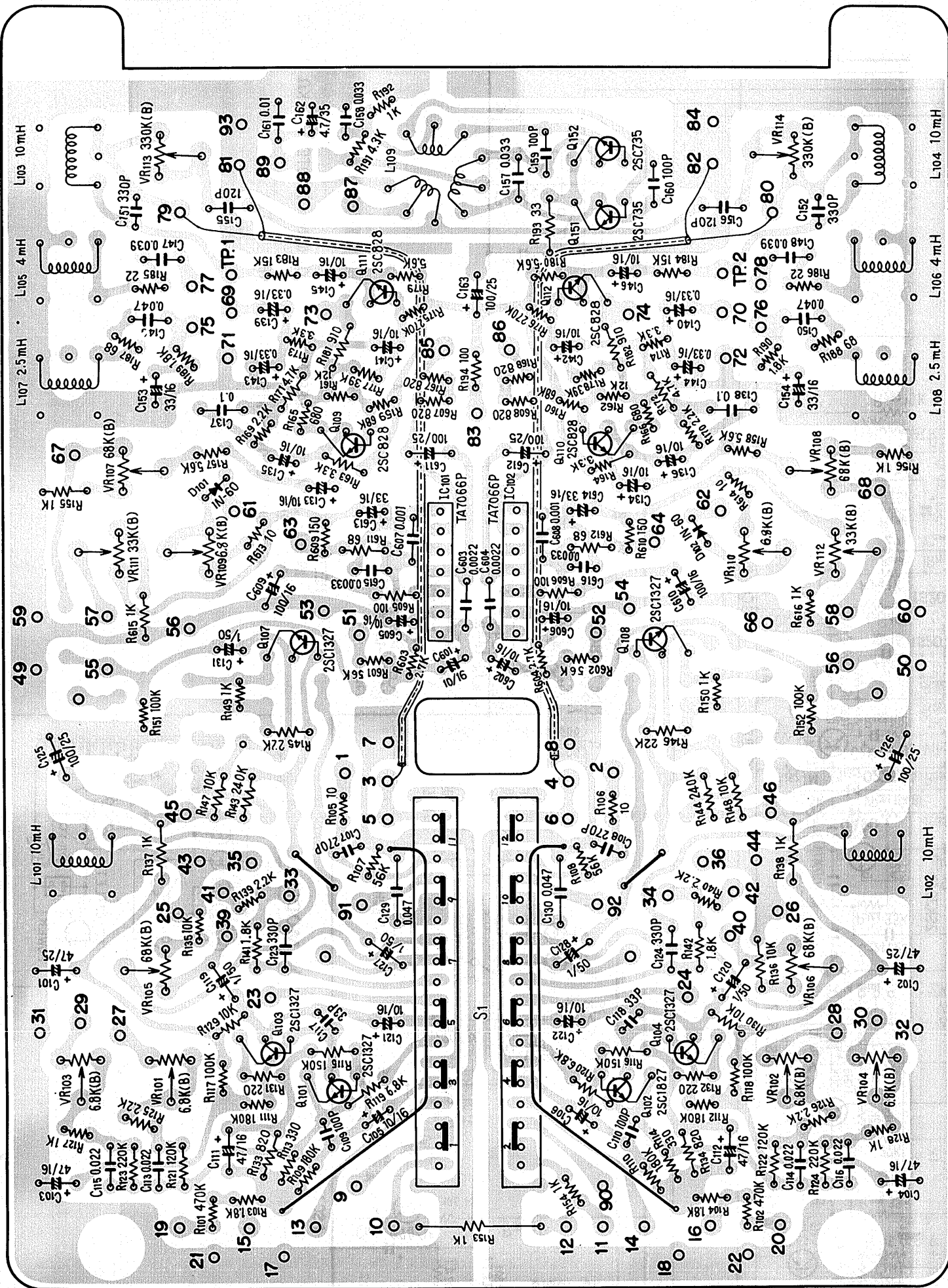
REC/PB amp ass'y RWF-039
