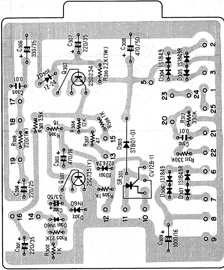
Sensing circuit ass'y RWR-023
