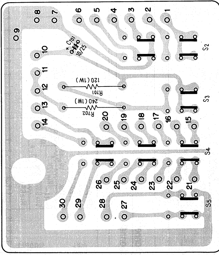
Switch circuit ass'y RWS-022
