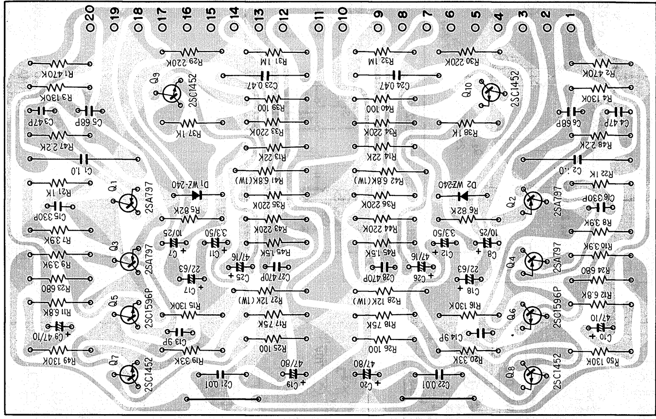
Flat amp ass'y A AWG-026
