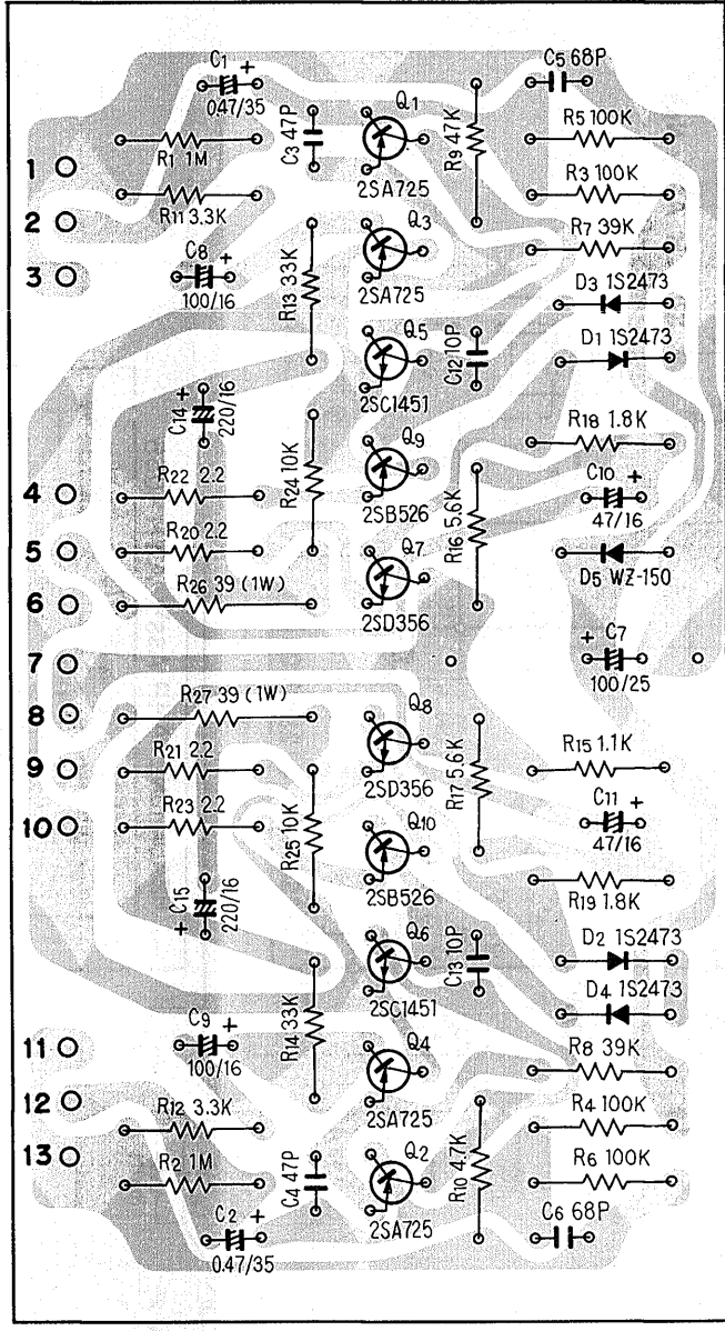
Headphone amp ass'y AWM-055
