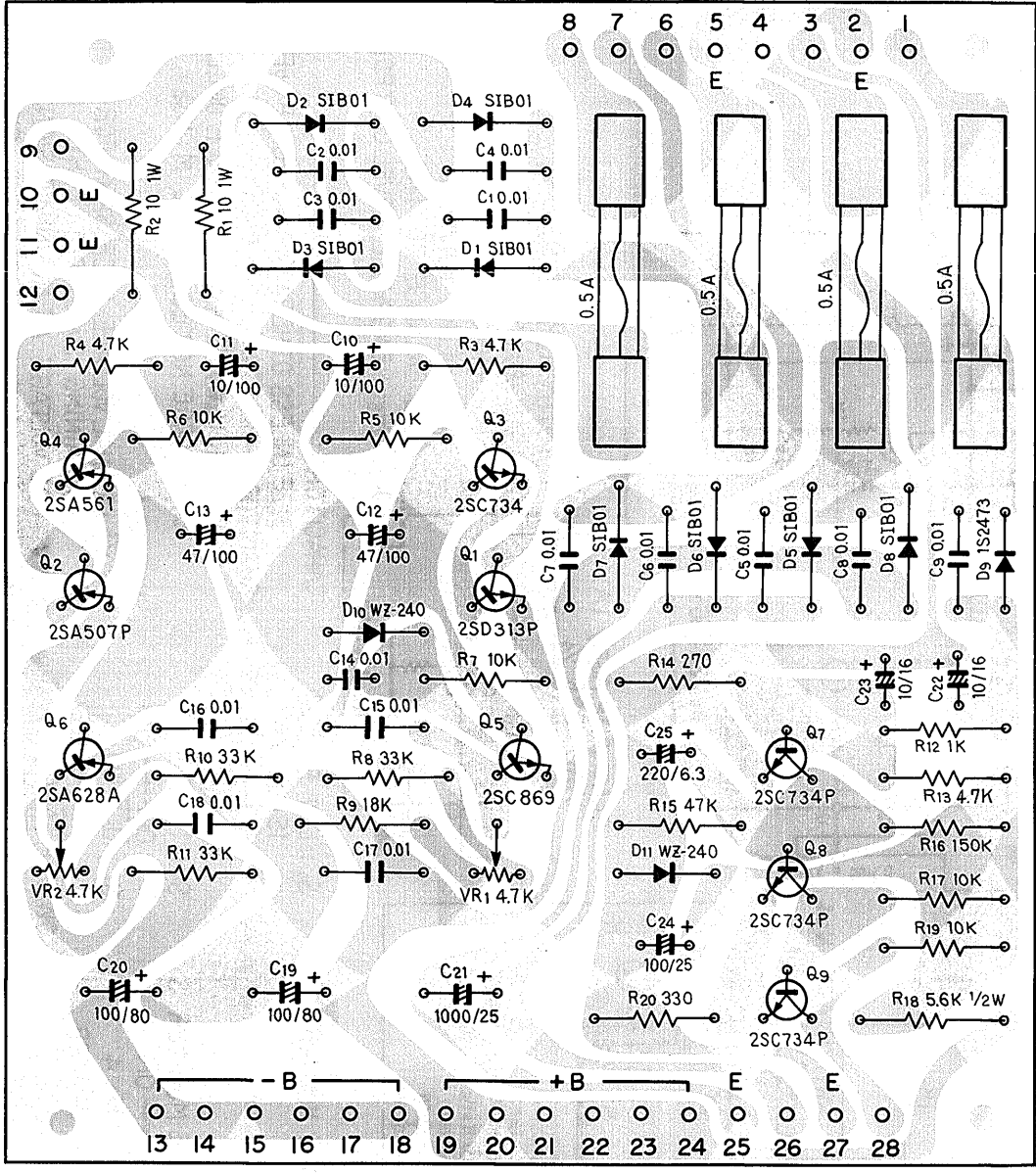
Power supply ass'y AWR-048
