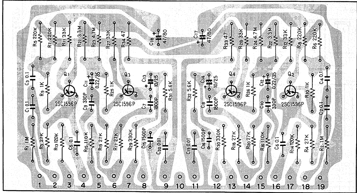
Filter amp ass'y AWM-053
