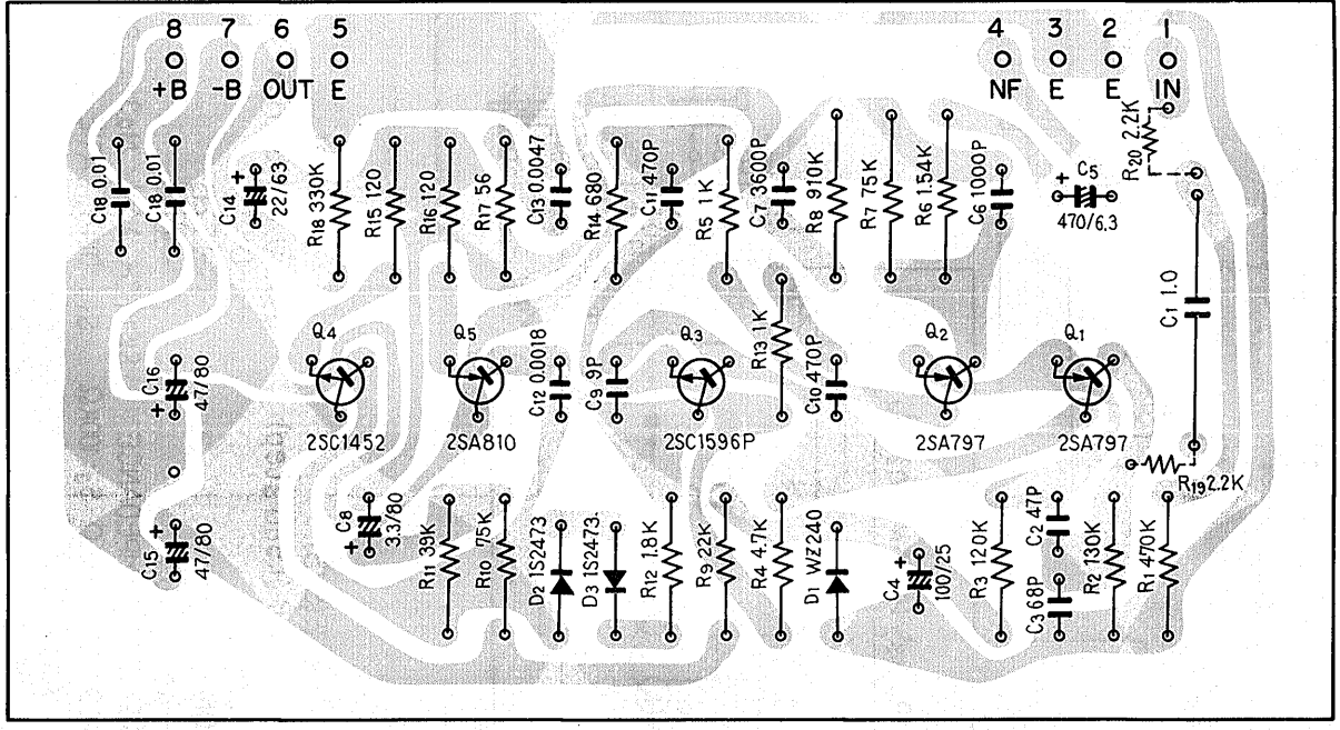
Equalizer amp ass'y AWF-012
