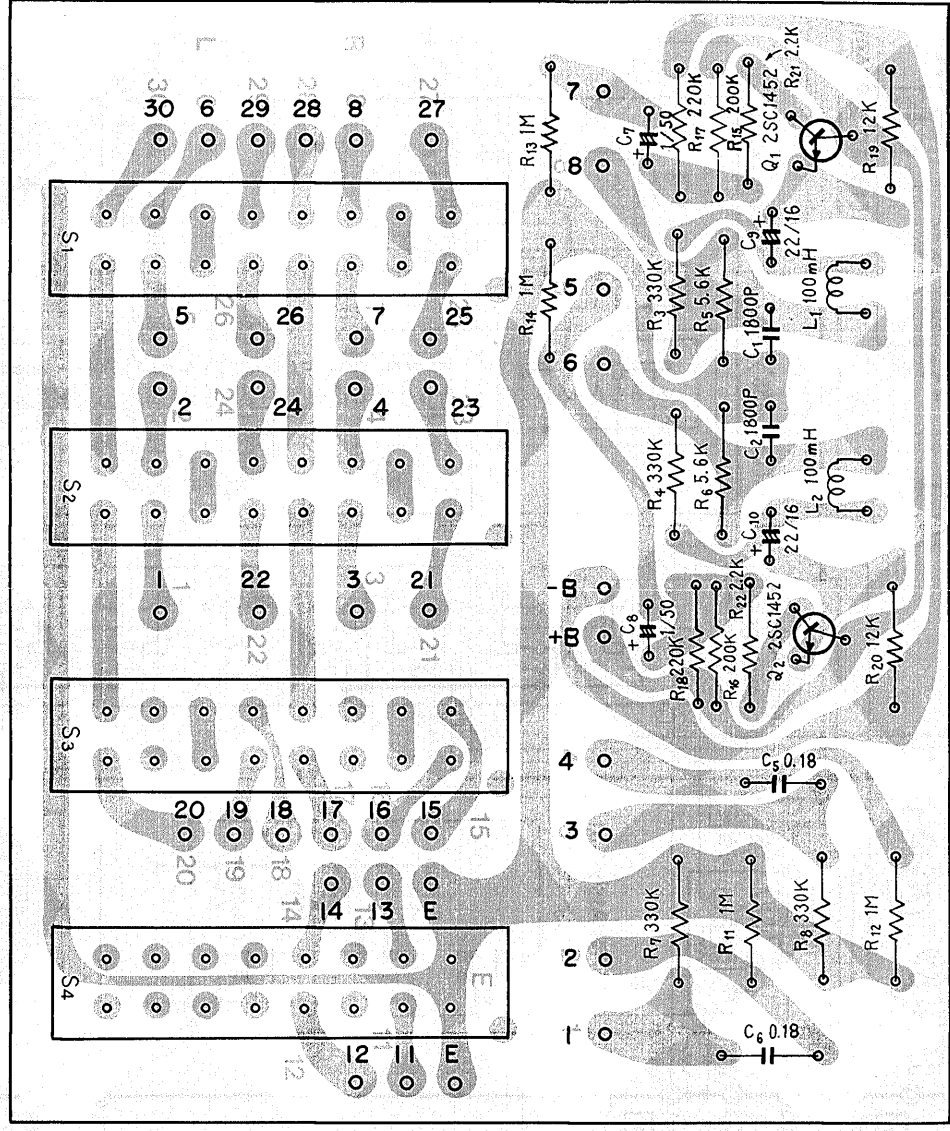
Switch ass'y No.4 AWS-057
