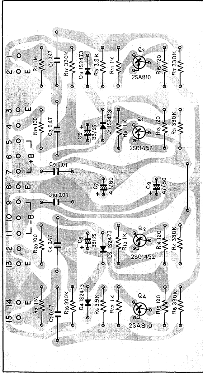
Buffer amp ass'y AWM-052
