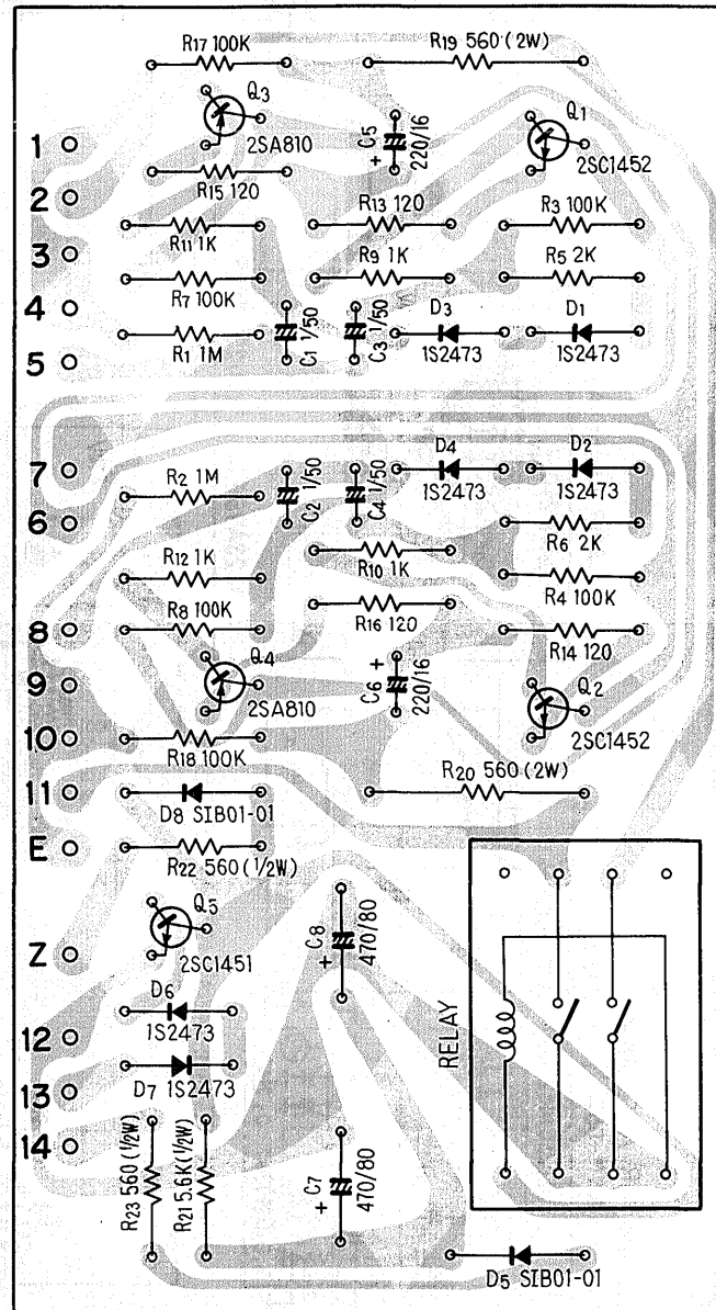
Muting buffer amp ass'y AWM-054
