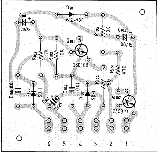
Power supply ass'y W16-021
