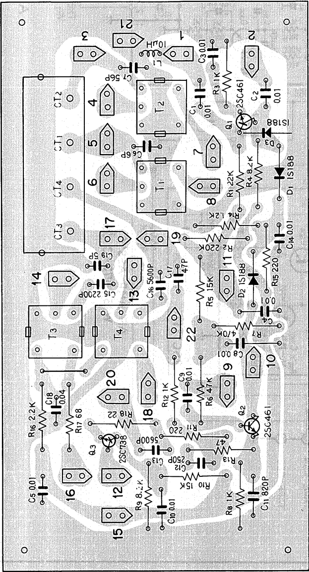
AM front end ass'y AWA-002
