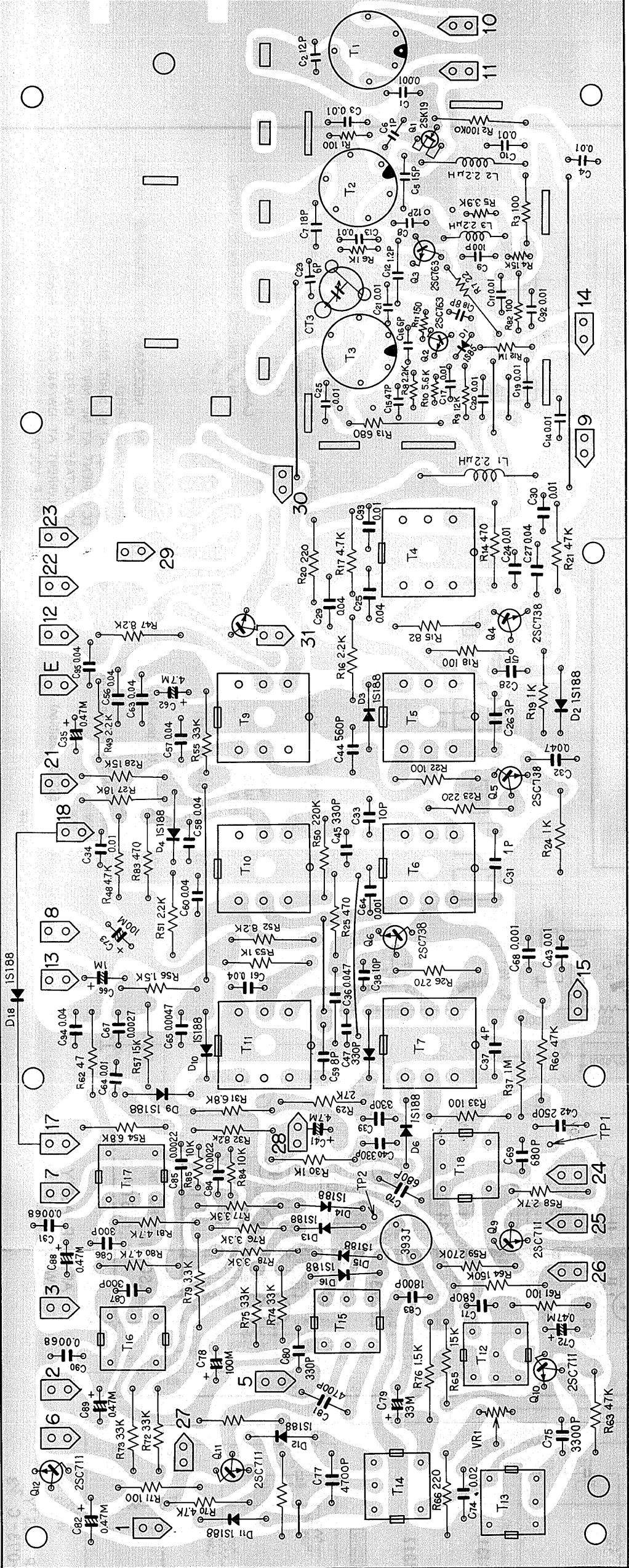
Tuner ass'y AWE-006
