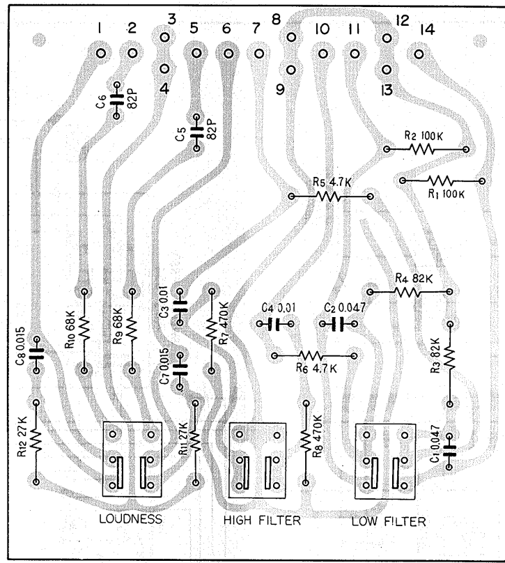
Switch circuit ass'y AWS-034
