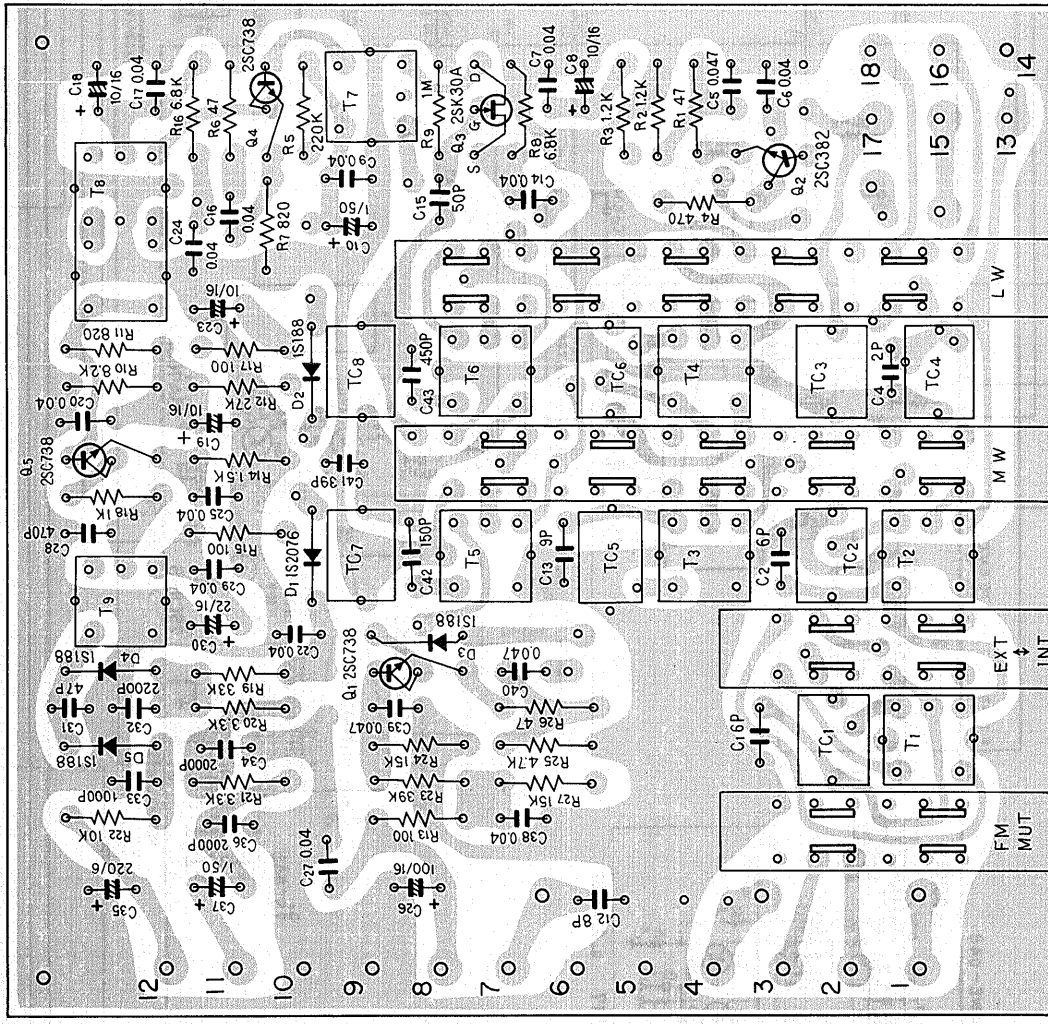
LW, MW tuner ass'y AWA-005
