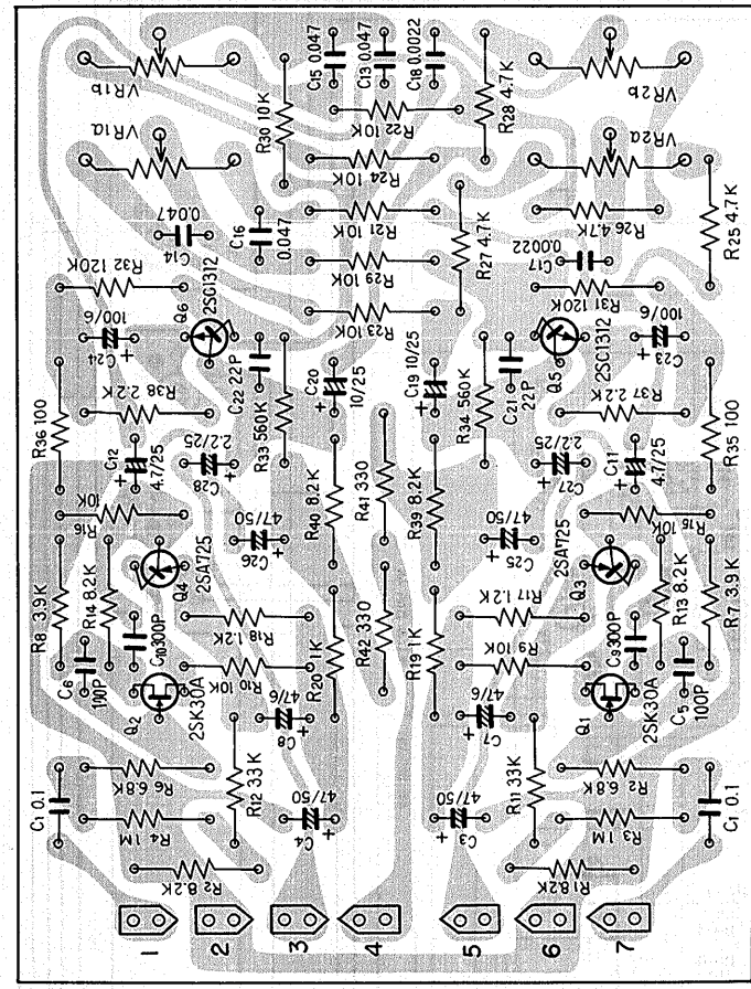
Control amp ass'y AWW-008
