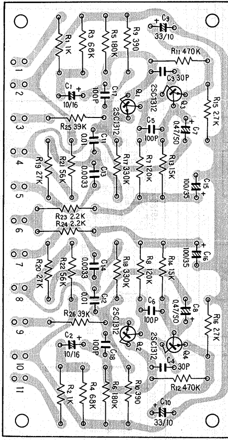
Equalizer amp ass'y W21-004
