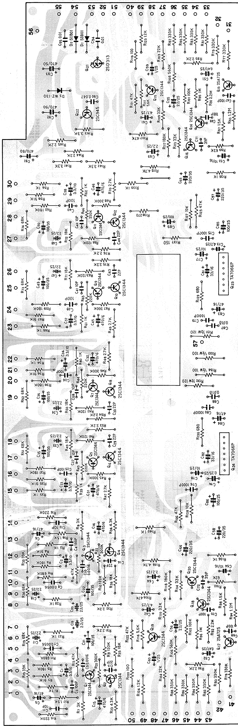
MIC amp ass'y AWM-056
