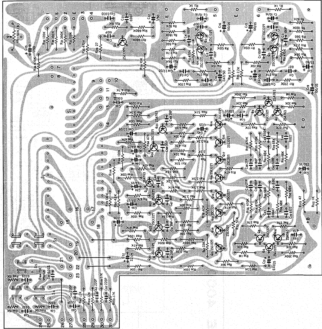
AF amp ass'y AWK-022
