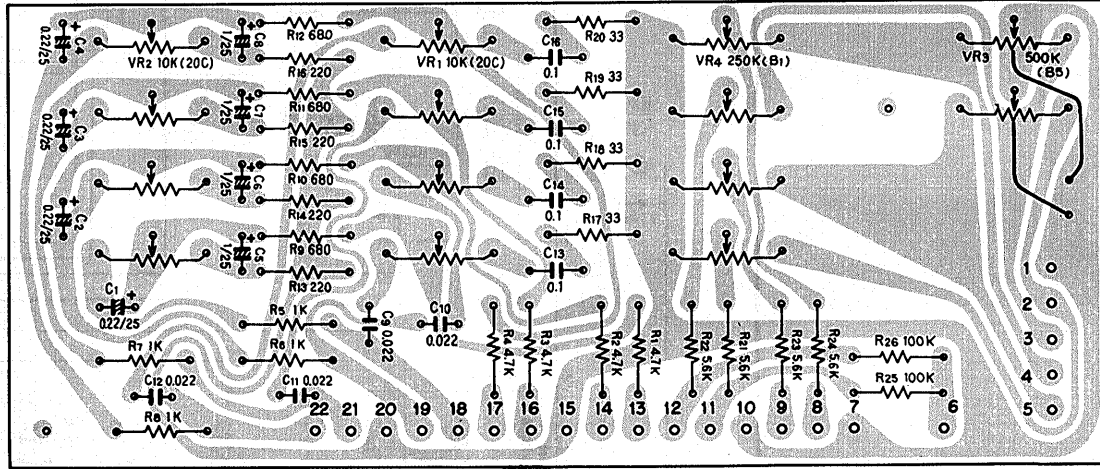
Control amp ass'y AWG-019
