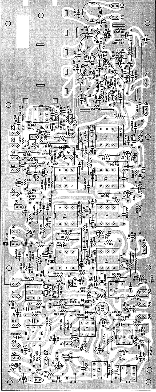
Tuner ass'y KWE-803 MSA model
