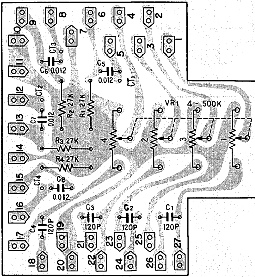
Volume ass'y AWX-001
