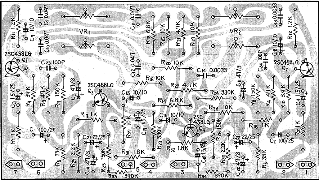
Control amp ass'y AWG-001
