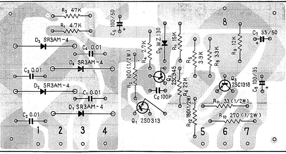
Power supply ass'y AWR-018
