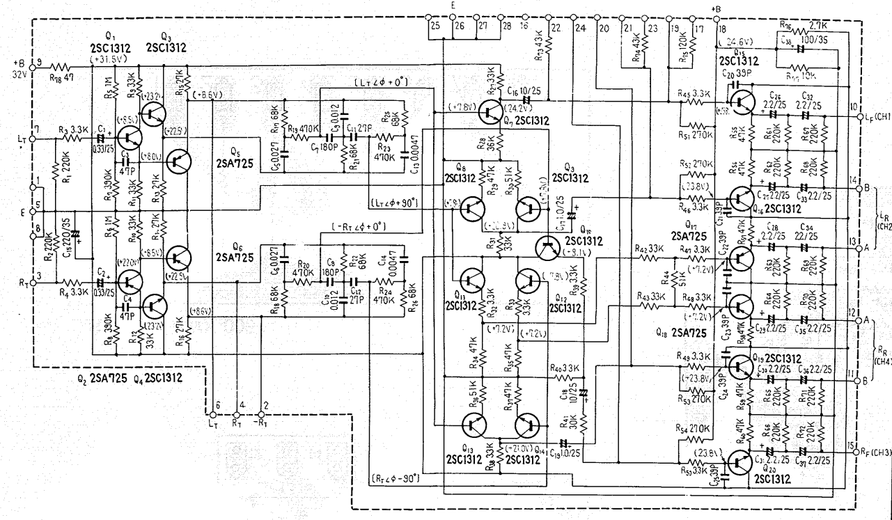
Decoder ass'y AWM-031
