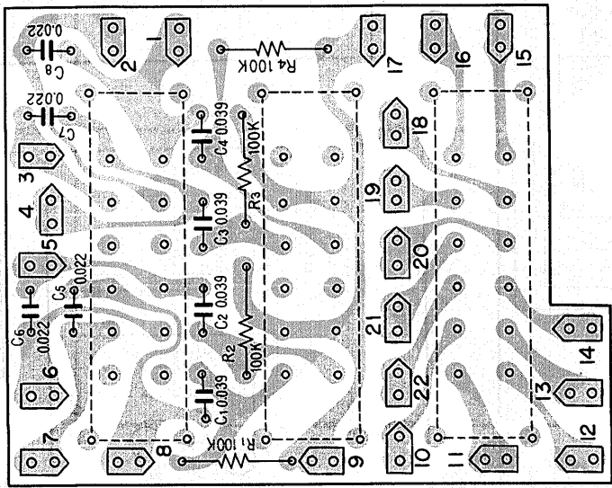
Switch ass'y AWS-003
