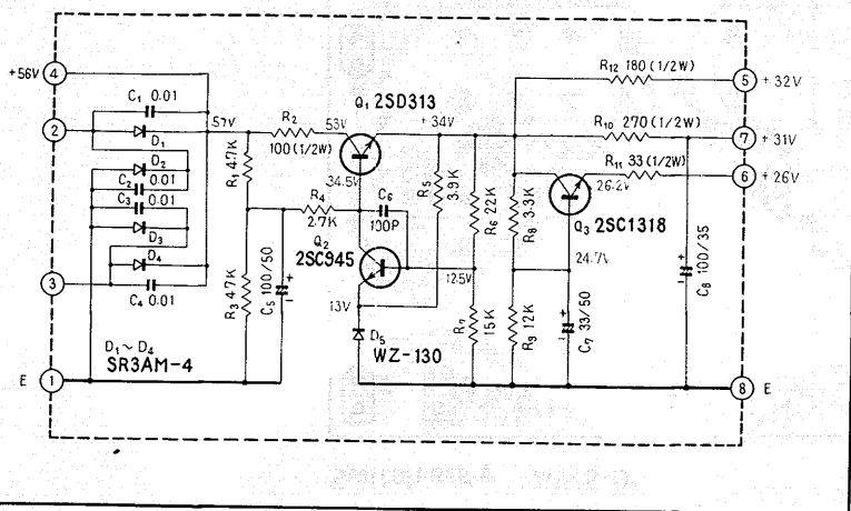
Power supply ass'y AWR-018
