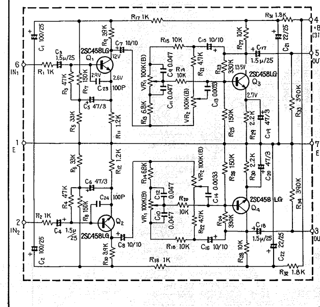
Control amp ass'y AWG-001
