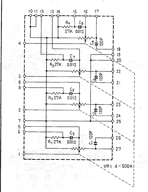
Volume ass'y AWX-001
