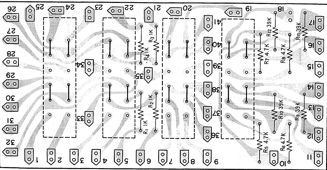
Switch ass'y AWS-002
