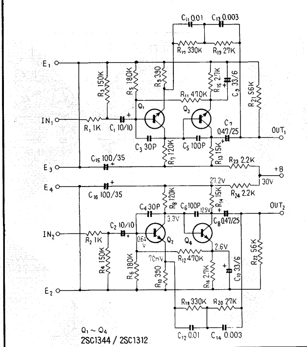
Head amp ass'y W15-032
