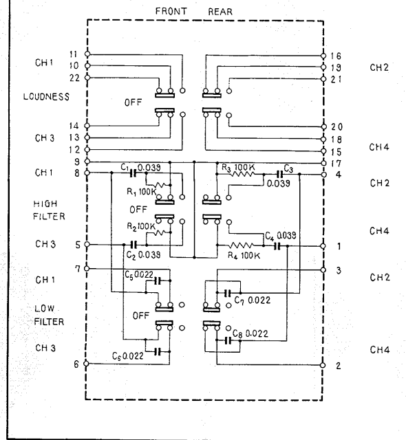
R ass'y AWX-005
