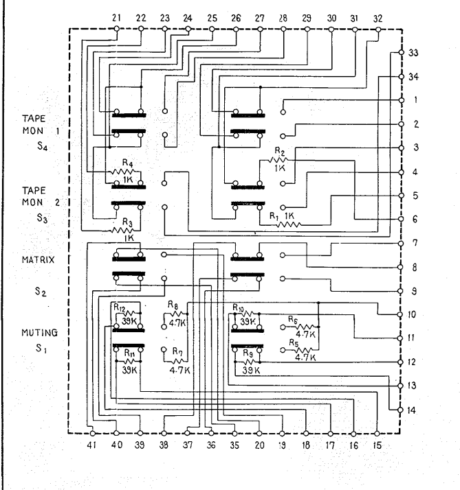
Switch ass'y AWS-002
