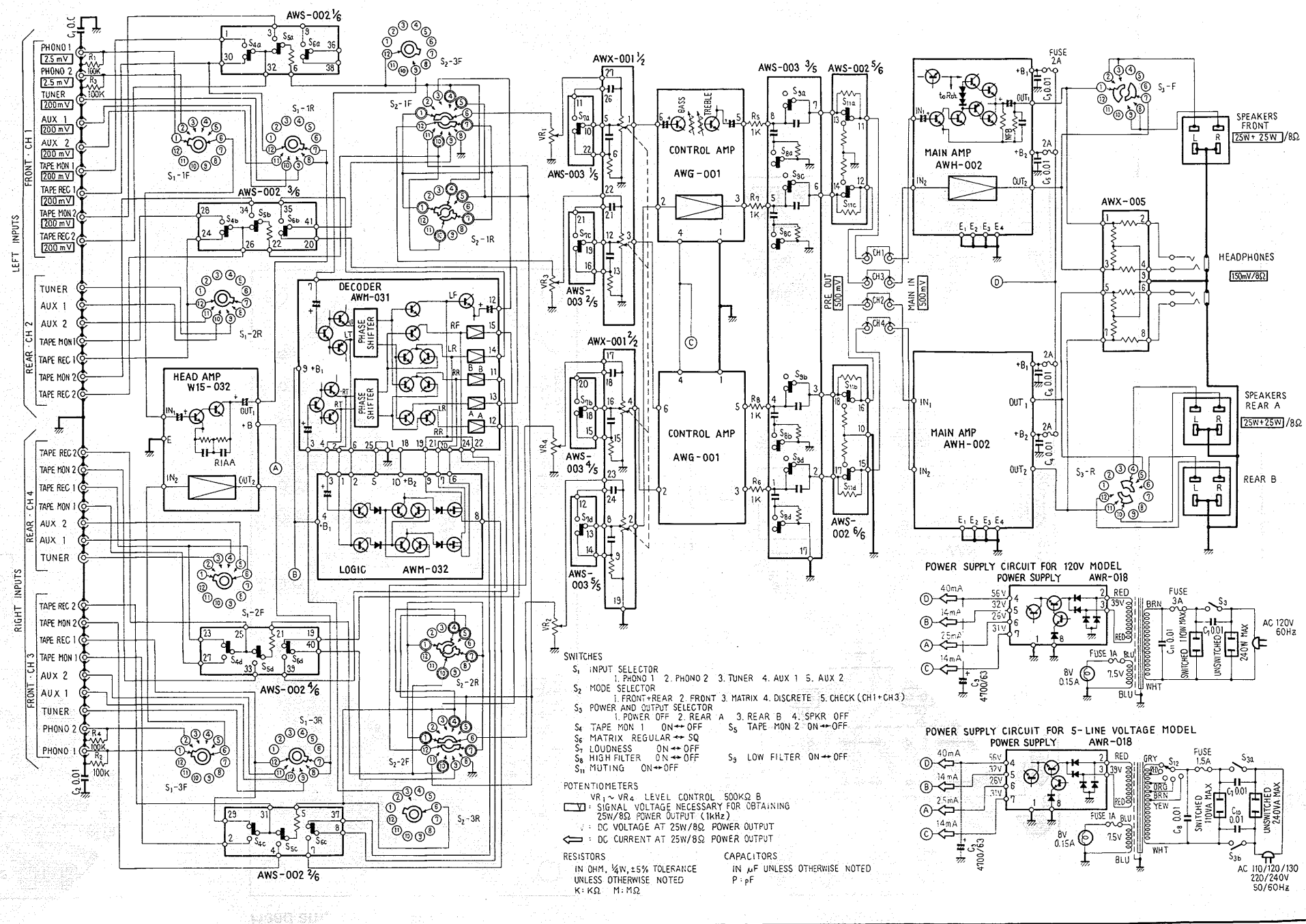
Decoder ass'y AWM-031
