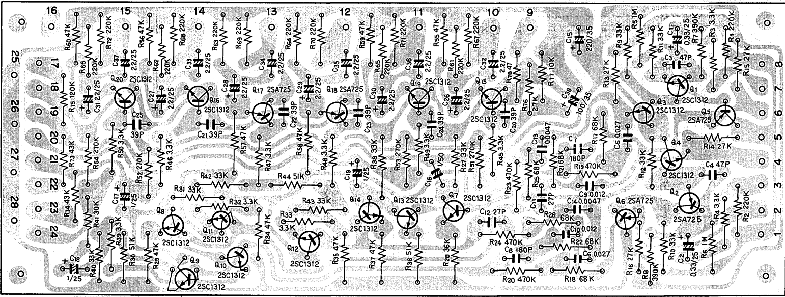
Decoder ass'y AWM-031
