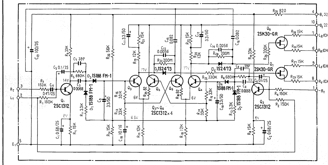
Logic ass'y AWM-032
