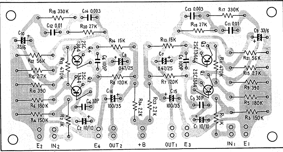
Head amp ass'y W15-032
