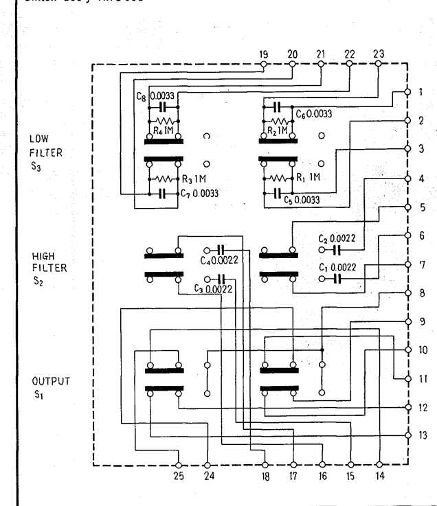
Switch ass'y AWS-001
