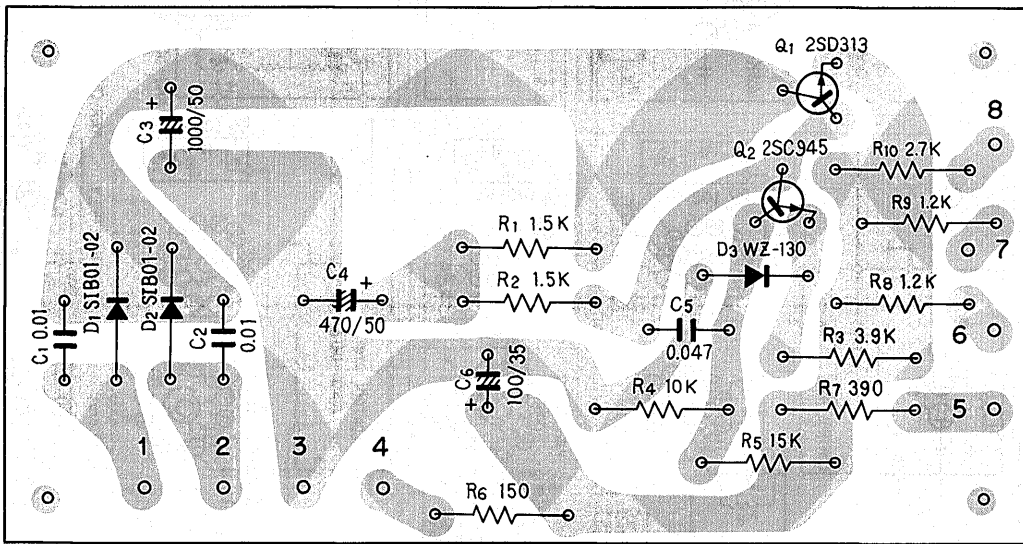
Power supply ass'y AWR-019
