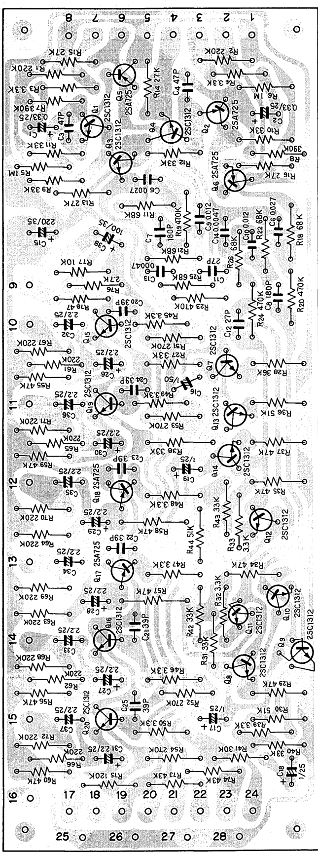
Decoder ass'y AWM-031
