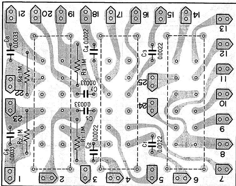
Switch ass'y AWS-001
