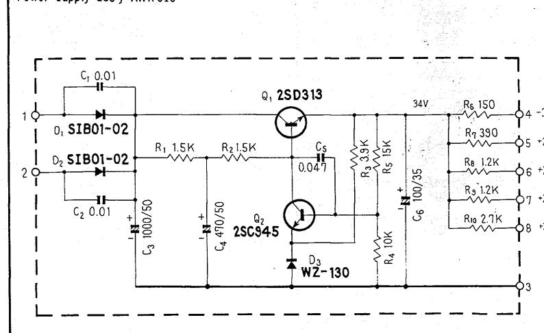
Power supply ass'y AWR-019
