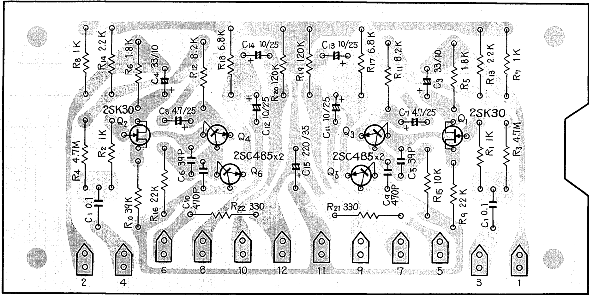
Control amp ass'y AWG-002
