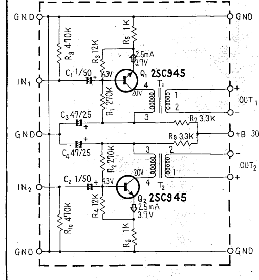
Headphone amp ass'y AWK-016
