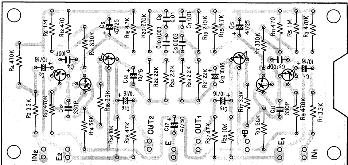
Head amp ass'y AWF-002
