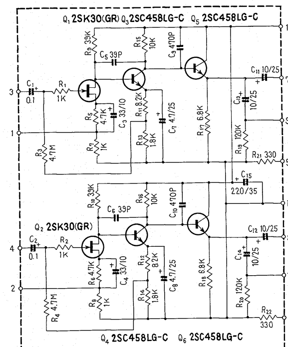
Control amp ass'y AWG-002
