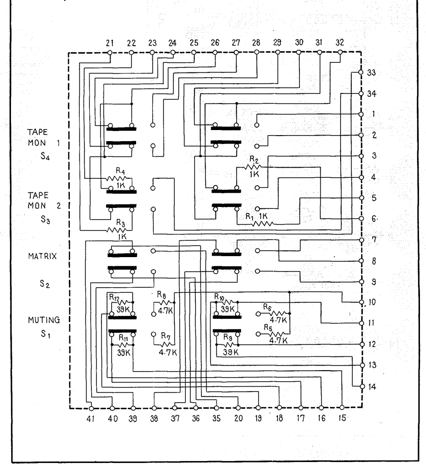
Switch ass'y AWS-002
