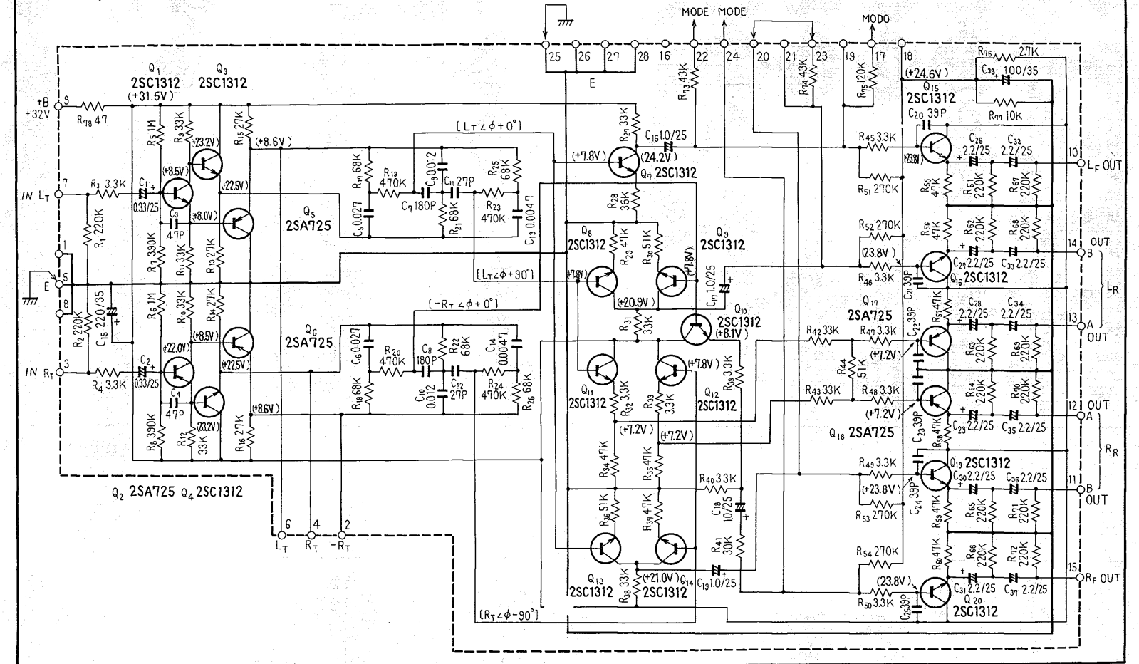
Decoder ass'y AWM-031
