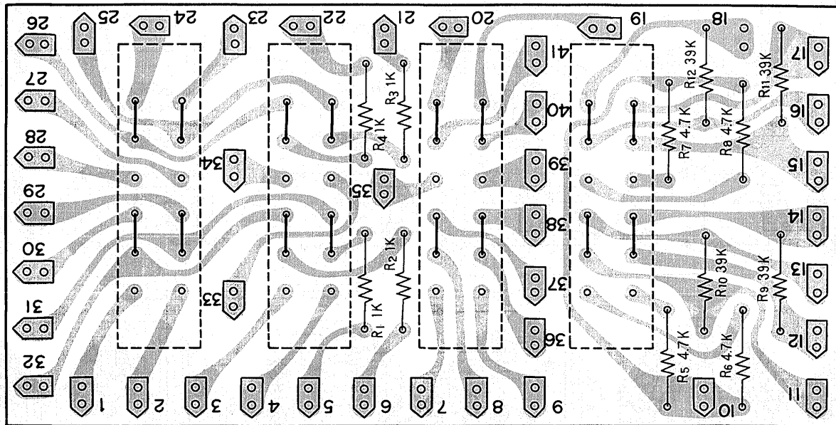
Switch ass'y AWS-002
