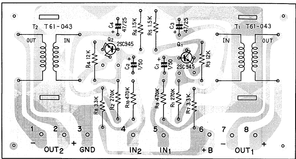
Headphone amp ass'y AWK-016
