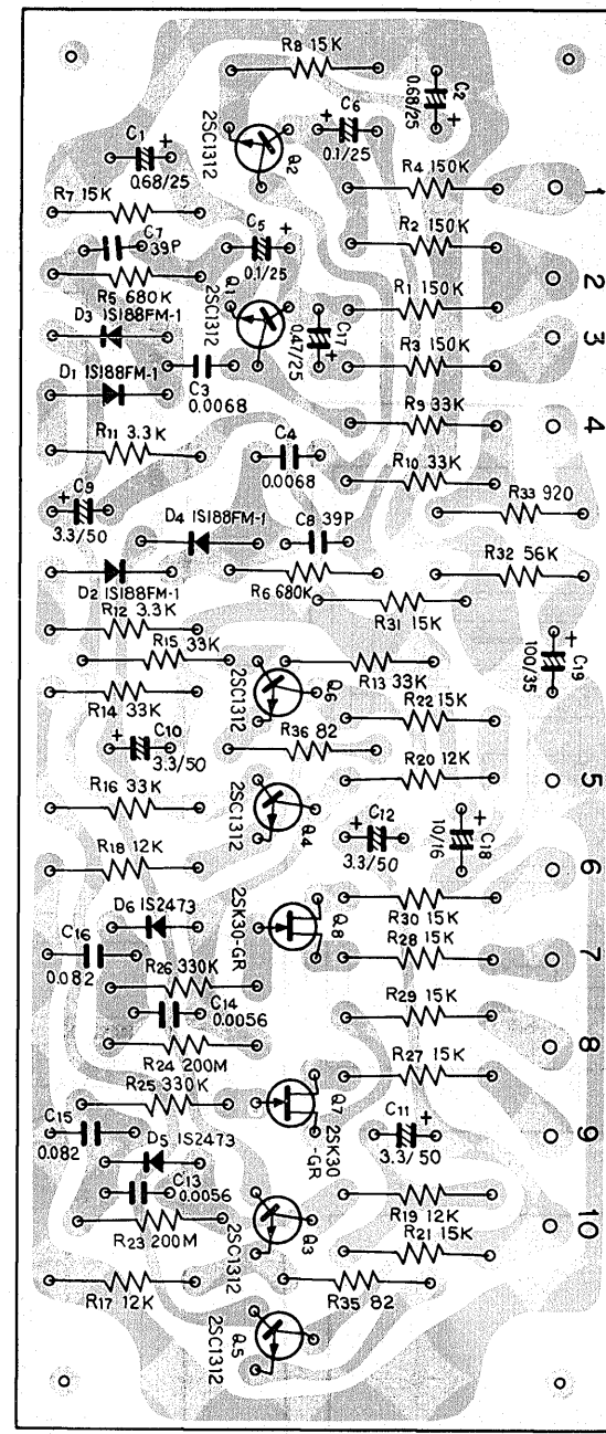
Logic ass'y AWM-032
