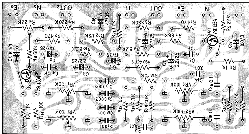
Control amp ass'y AWM-009
