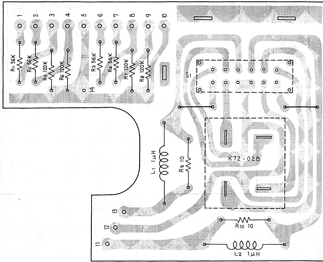
Input and output ass'y AWM-026
