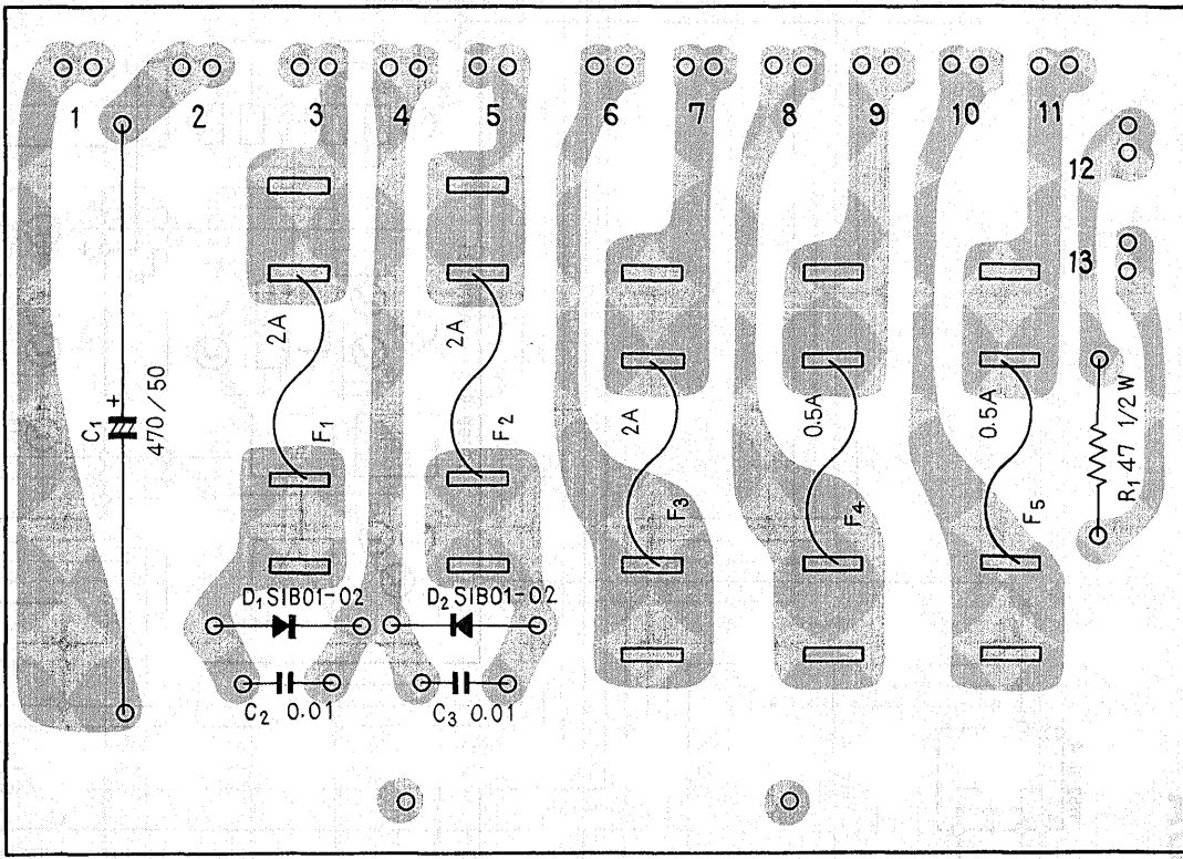
Power supply ass'y AWR-016
