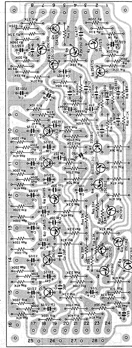
Decoder ass'y AWM-065
