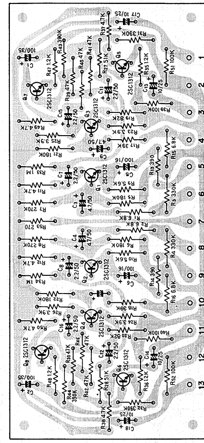
Matrix ass'y AWM-048
