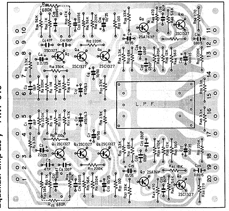
Equalizer amp ass'y AWF-010
