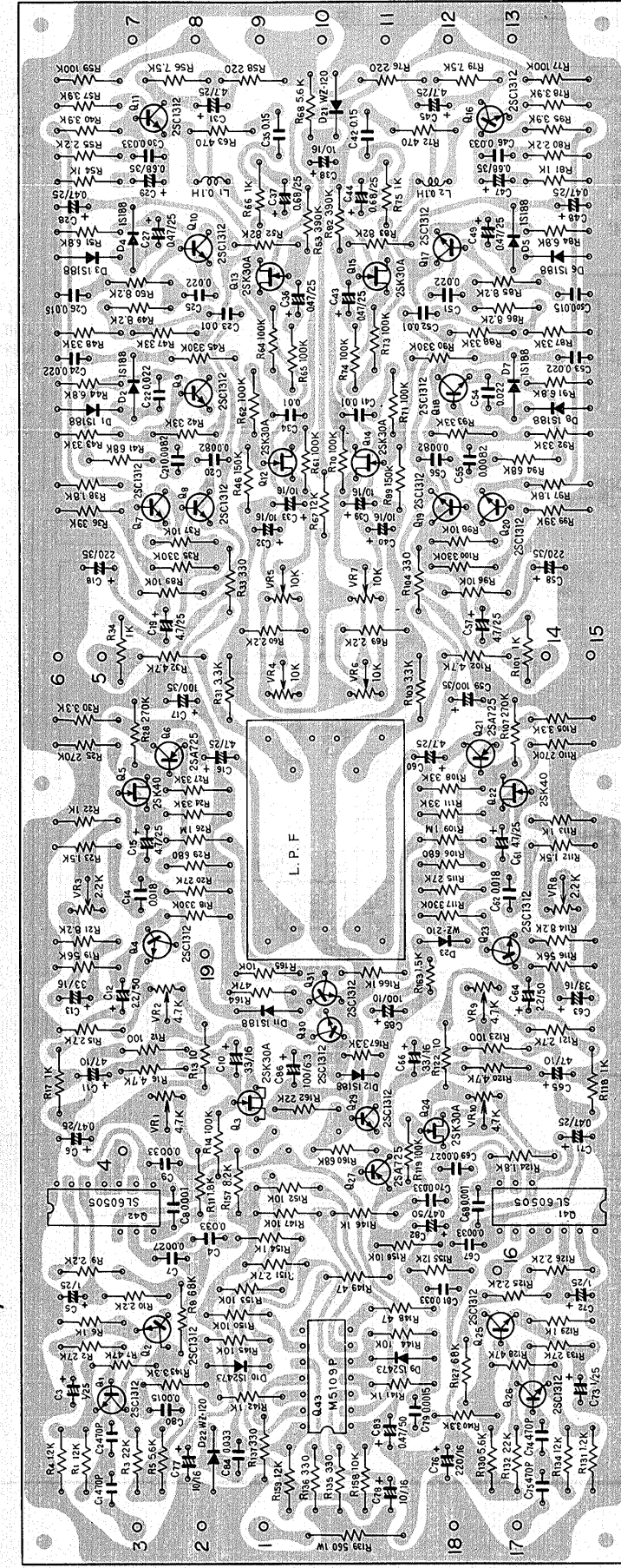
Sub channel circuit ass'y AWX-051
