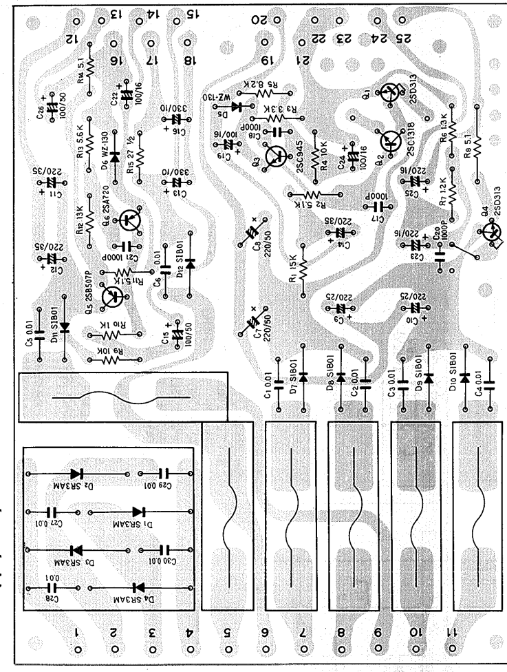
Power supply ass'y AWR-040
