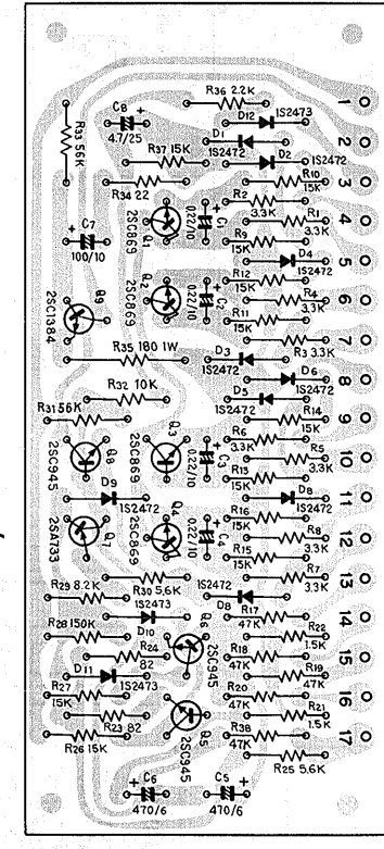
Protection circuit ass'y AWM-049
