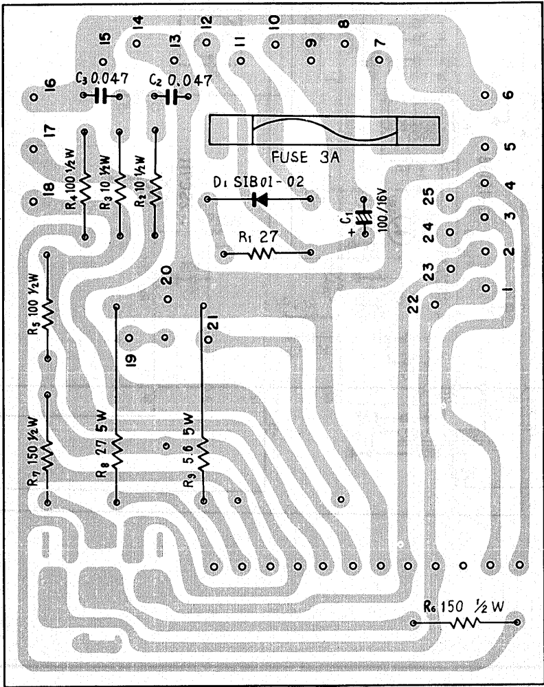
Switch circuit ass'y KWS-801
