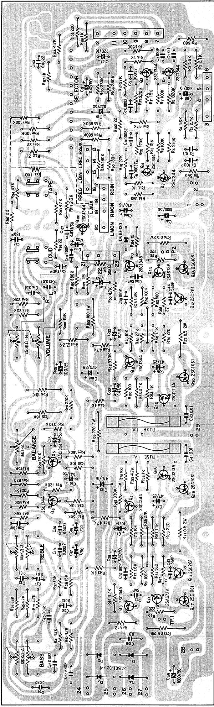
AF amp ass'y KWK-802
