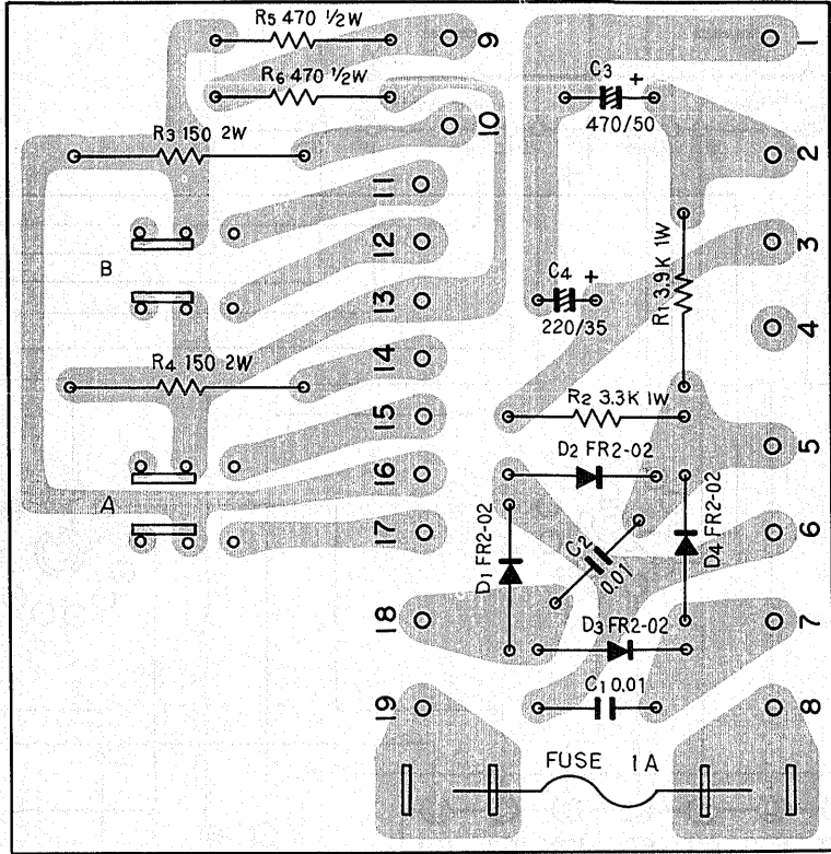
Switch circuit ass'y B AWS-044
