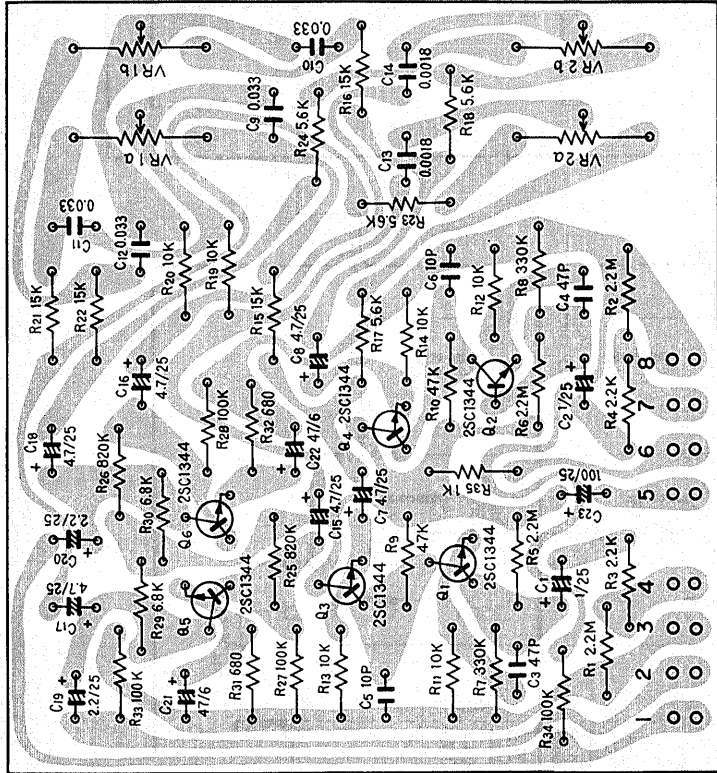
Control amp ass'y AWG-020
