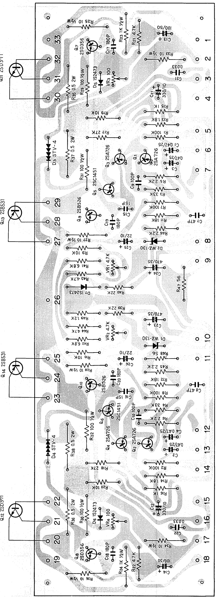
Power amp ass'y AWH-021
