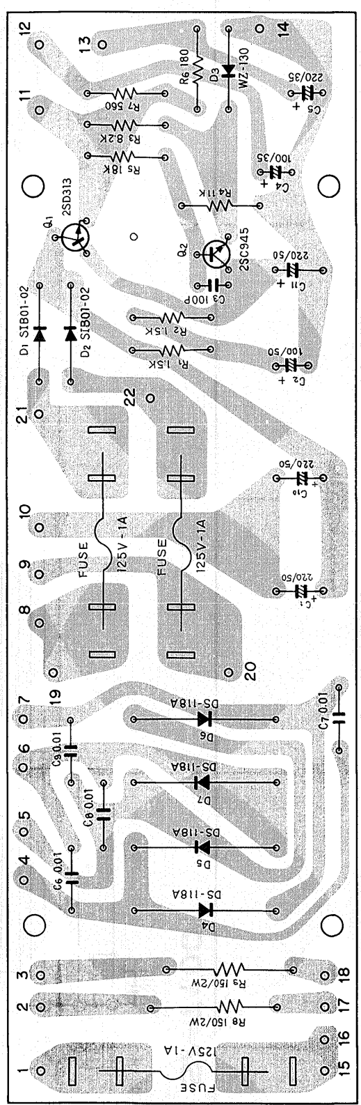
Power supply ass'y AWR-026
