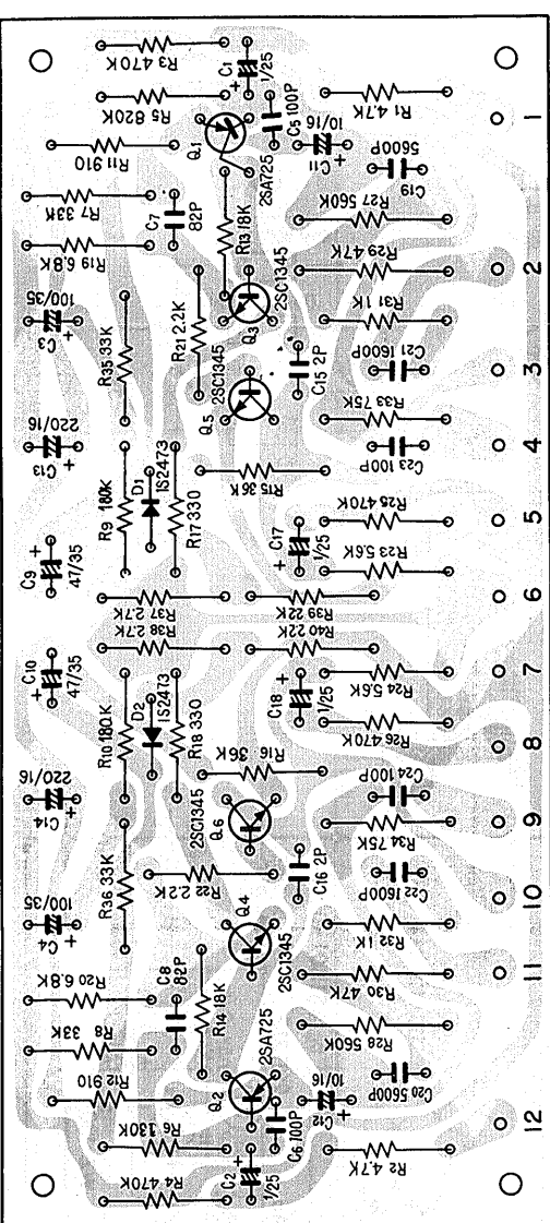
Equalizer amp ass'y AWF-005
