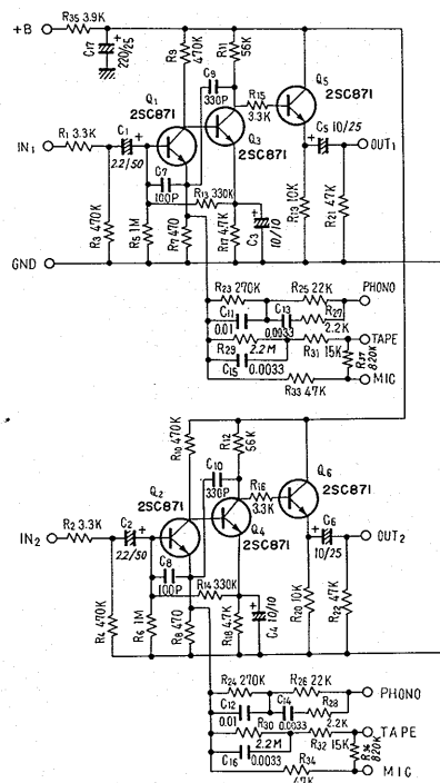
HEAD AMP UNIT W15-056
