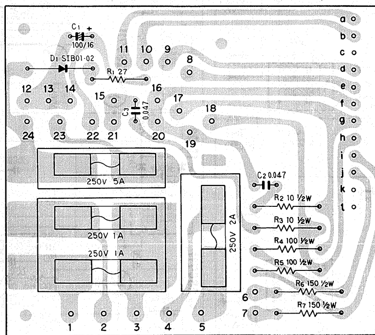
Power switch ass'y AWS-051 (NBW model)
