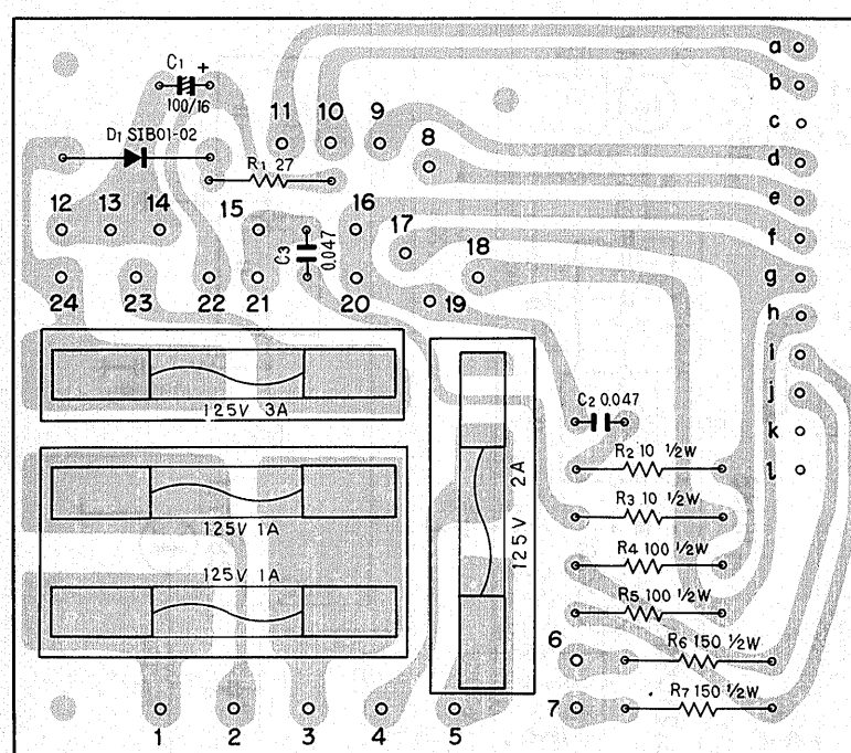
Power switch ass'y AWS-052 (FVW model)
