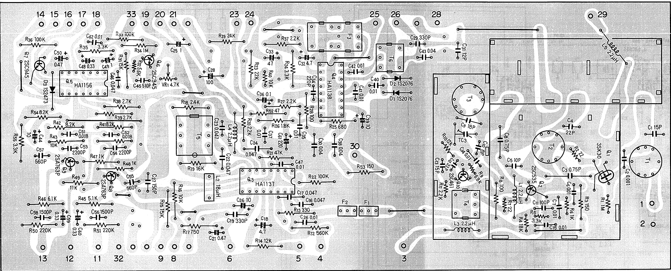
Tuner ass'y AWE-052
