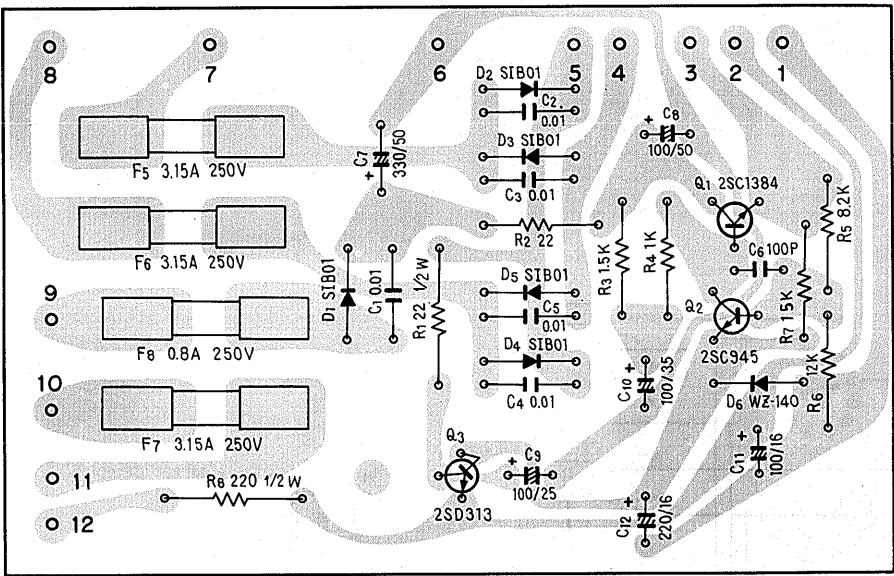
Power supply ass'y AWR-059 (GN model)
