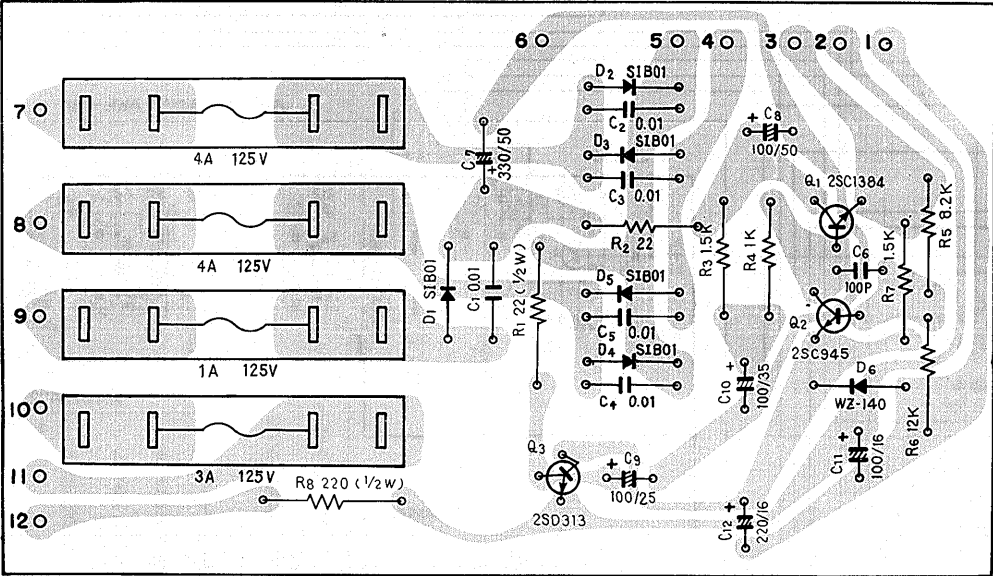
Power supply ass'y AWR-062 (FV, KCU model)
