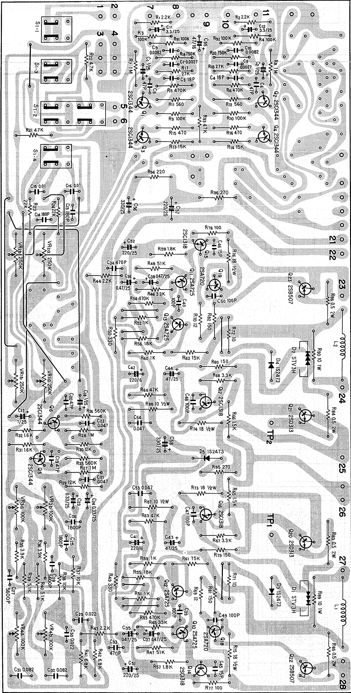
AF amp ass'y AWK-034
