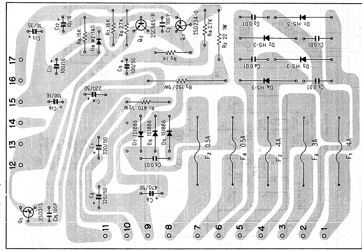
Power supply ass'y AWR-065
