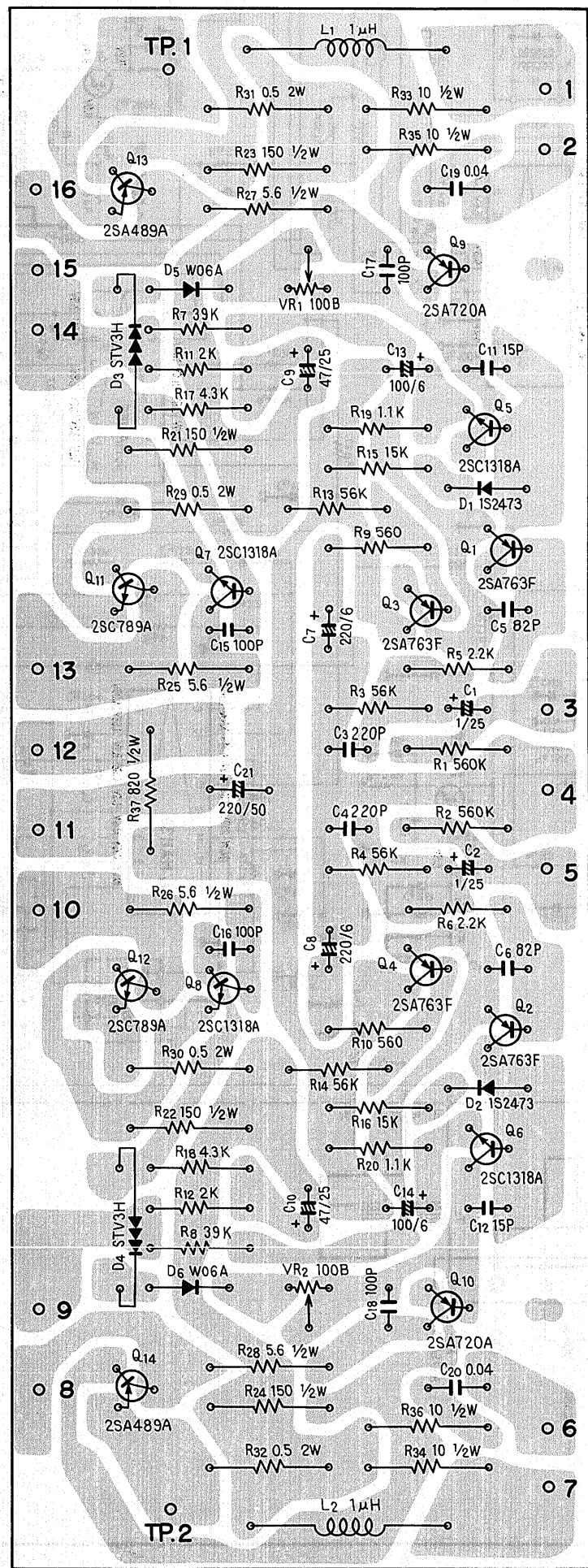
Power amp ass'y AWH-035
