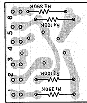
5P connector ass'y AWX-062
