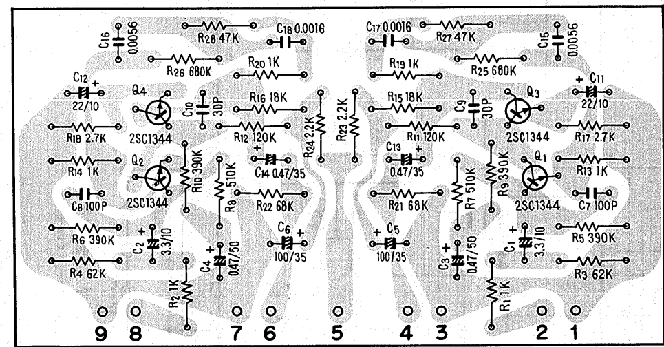
Equalizer amp ass'y AWF-014
