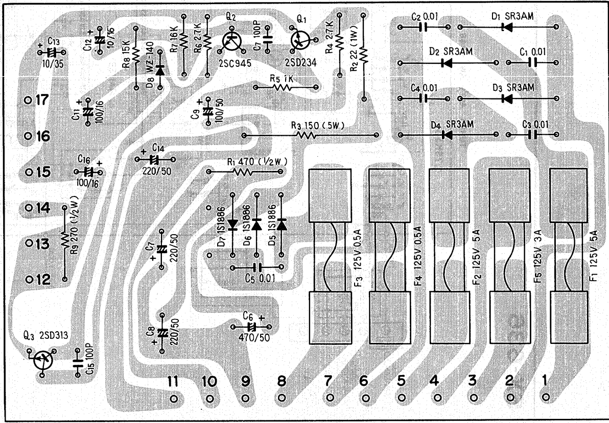
Power supply ass'y AWR-060 (FV, KCU model)
