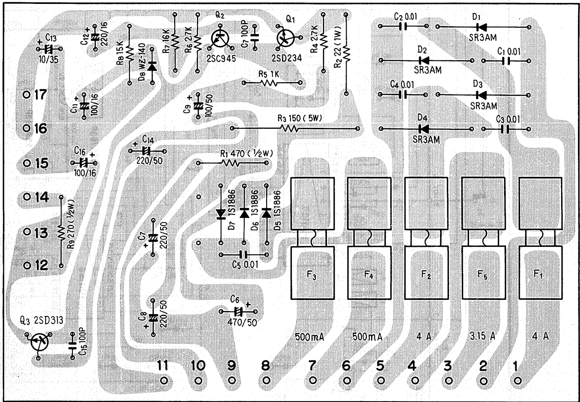
Power supply ass'y AWR-061 (GN model)
