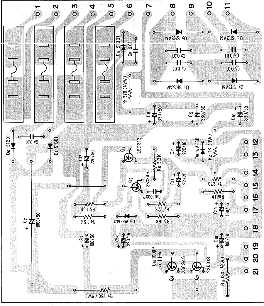
Power supply ass'y AWR-058 (GN model)
