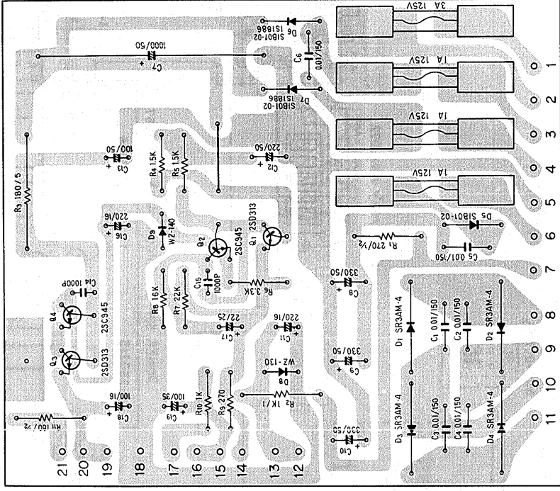
Power supply ass'y AWR-057 (F, KCU model)
