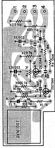
Mic amp ass'y AWM-066
