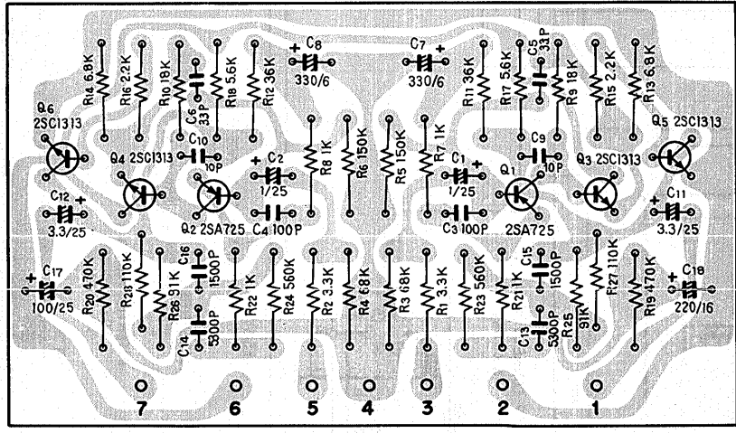
Equalizer amp ass'y AWF-011
