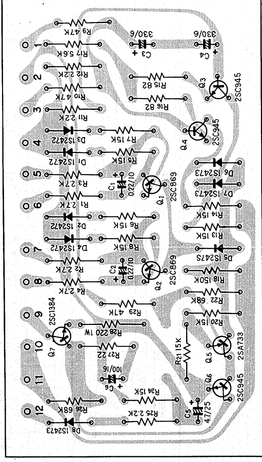
Protection ass'y AWM-025
