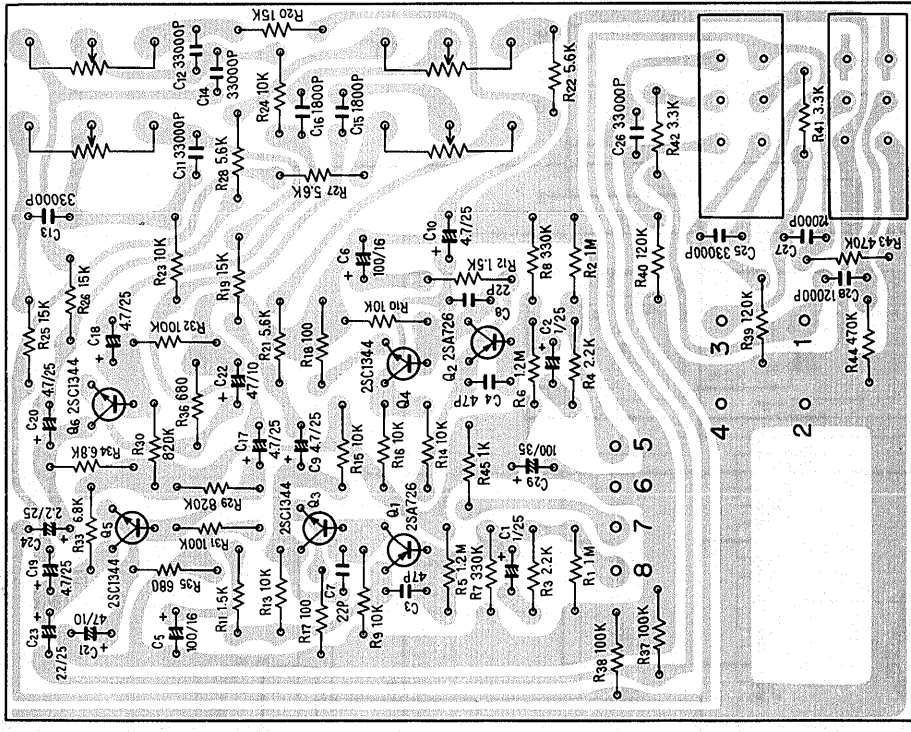
Control amp ass'y AWW-030
