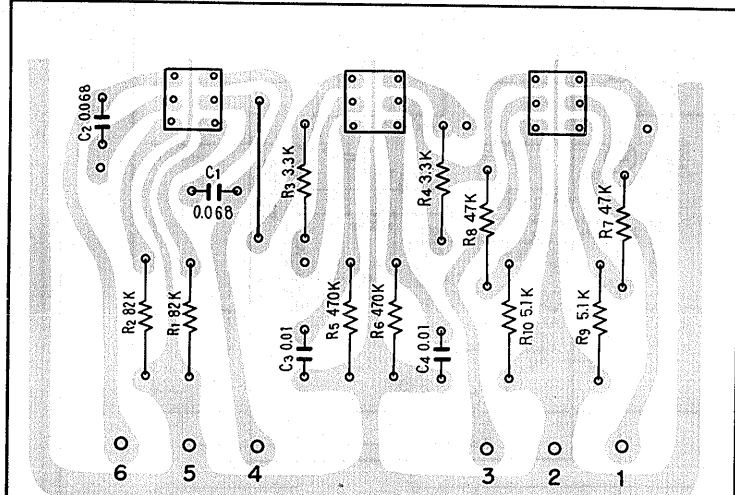
Filter and muting ass'y AWS-066
