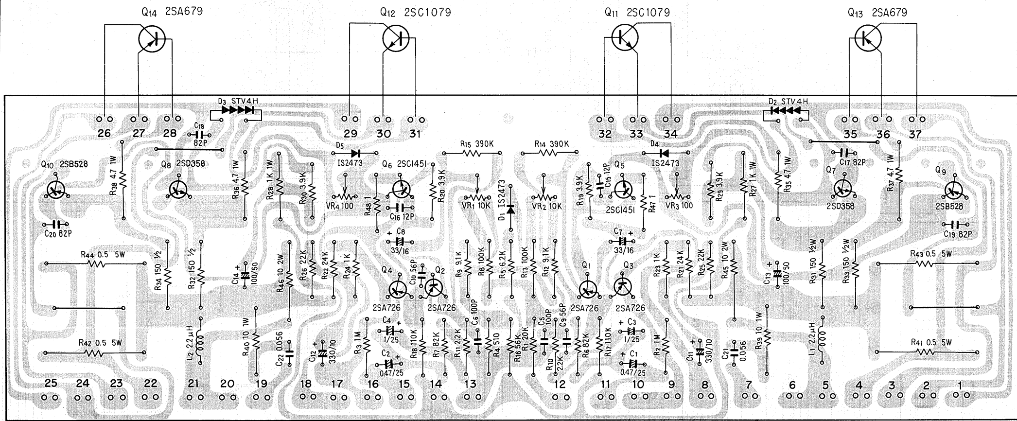
Power amp ass'y AWH-031
