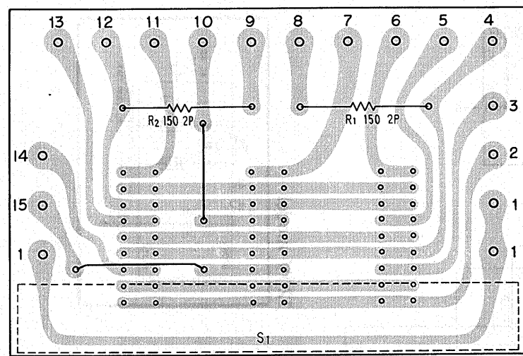
Switch circuit ass'y AWS-075
