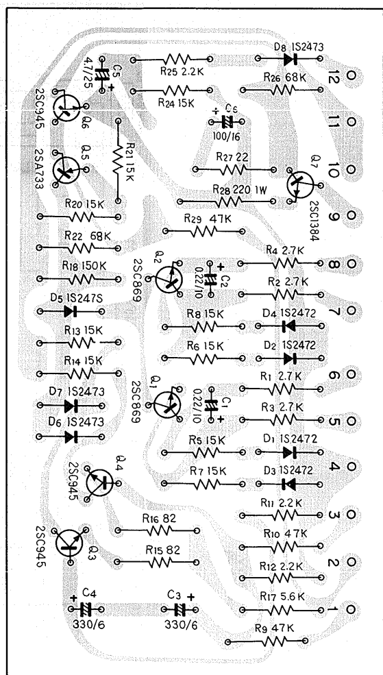
Protection circuit ass'y AWM-025
