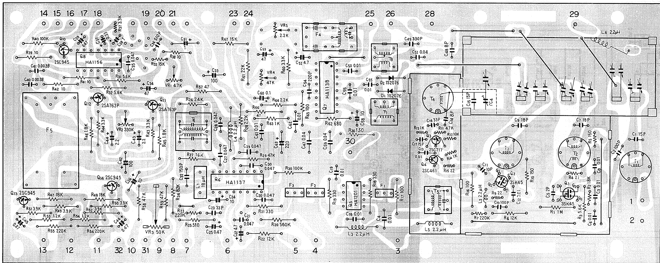
Tuner ass'y AWE-041
