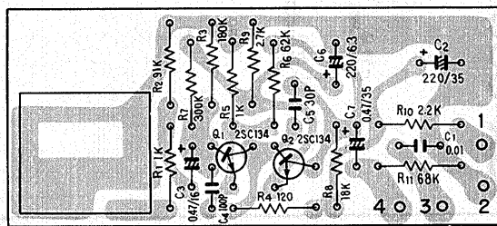
MIC amp ass'y AWM-064
