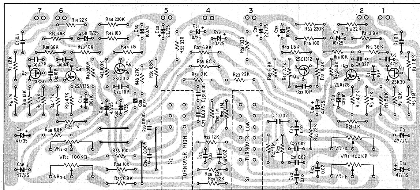
Control amp ass'y AWG-029
