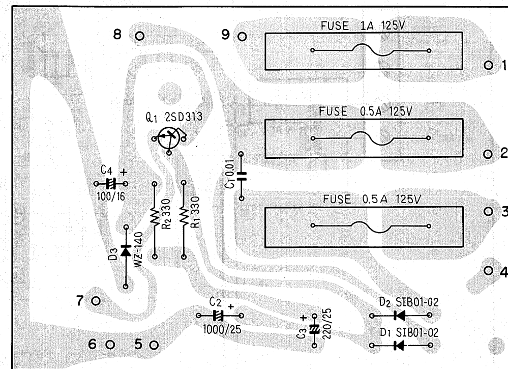
Power supply ass'y AWR-079 (FV model)
