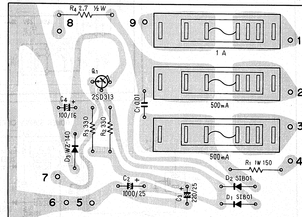
Power supply ass'y AWR-083 (GN model)
