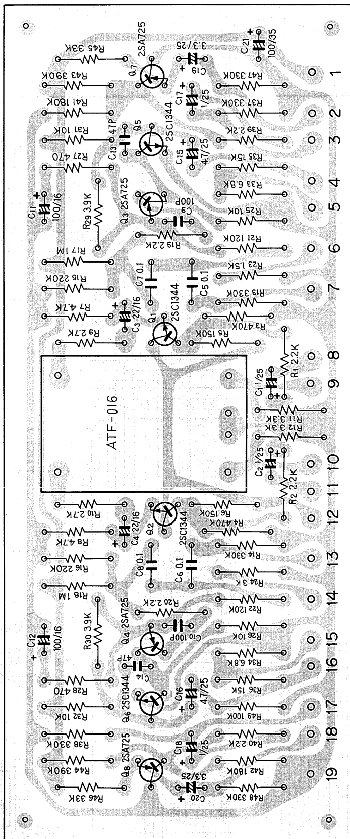
AF amp ass'y AWK-019
