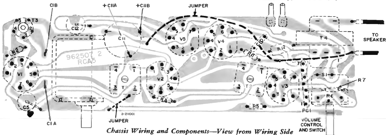
Chassis Wiring and Components—View from Wiring Side
