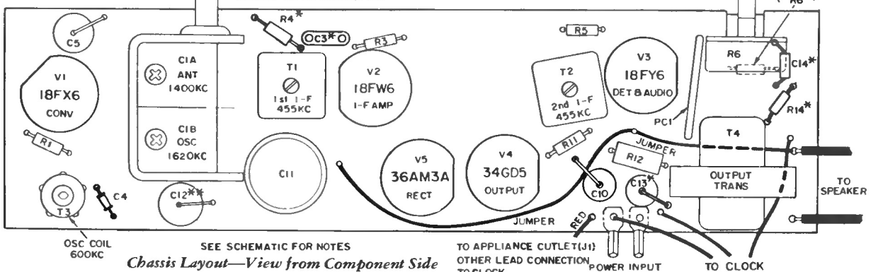
1-RD-4, -5, -6 R4 REPLACED BY JUMPER ON RC-1202 R, P & K
