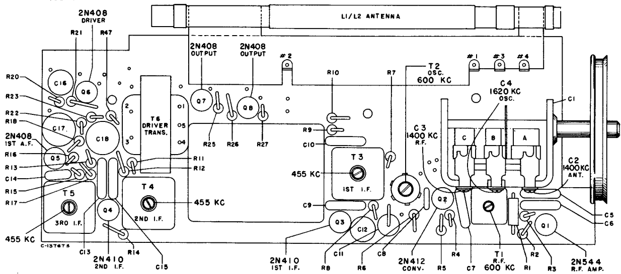
Transistor, Major Component and Trimmer Locations
