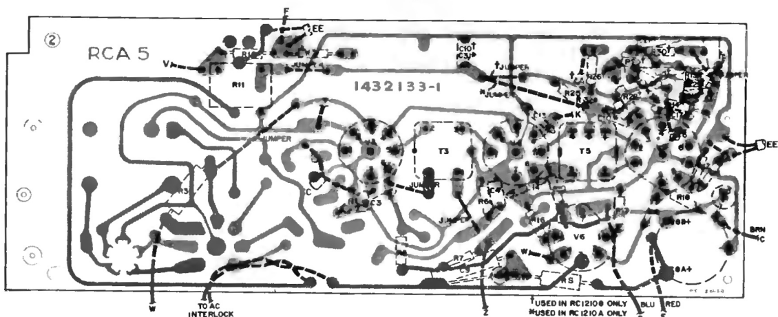
Chassis Wiring and Components—View from Wiring Side
