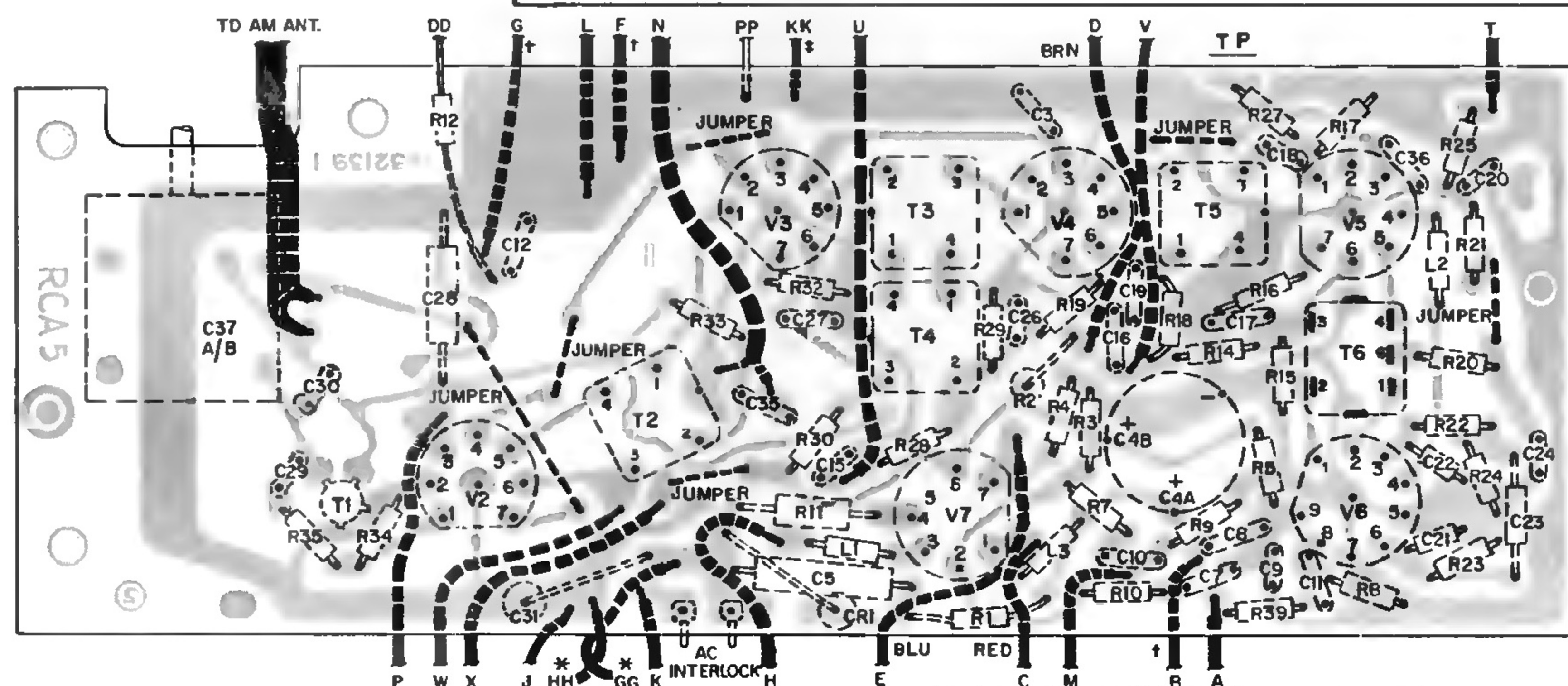
Chassis Wiring and Components—View from Wiring Side
