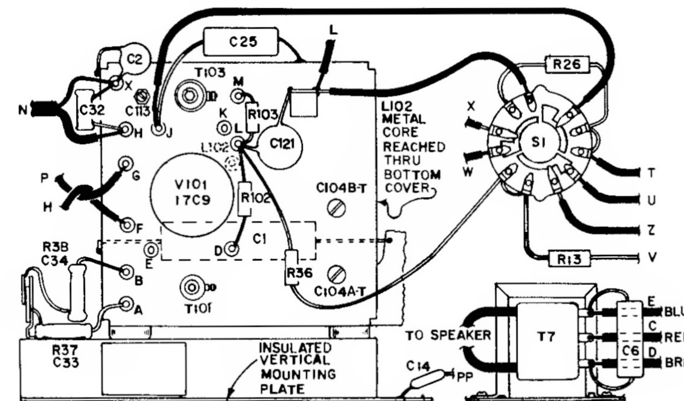
FM Tuner Layout
