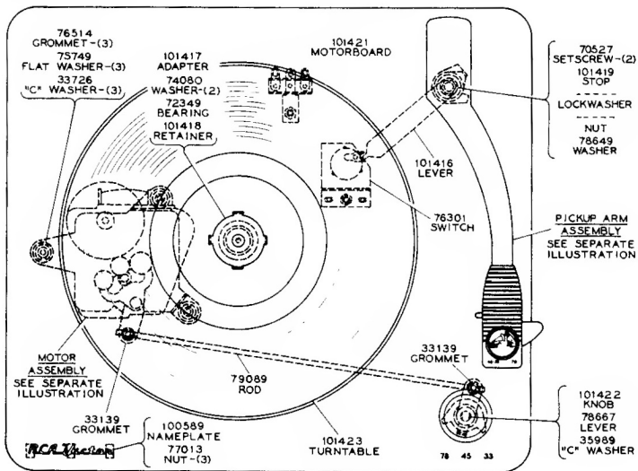
Motorboard Assembly
