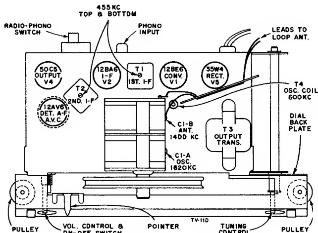
Tube and Trimmer Locations
