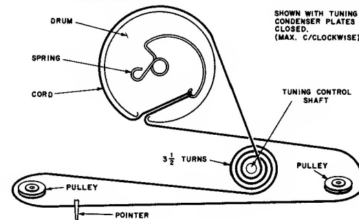
Tuning Drive Cord
