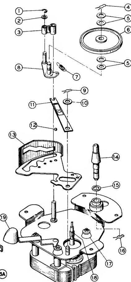
Motor Assembly
