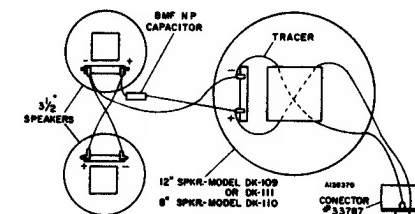
Speaker Connection Diagram
