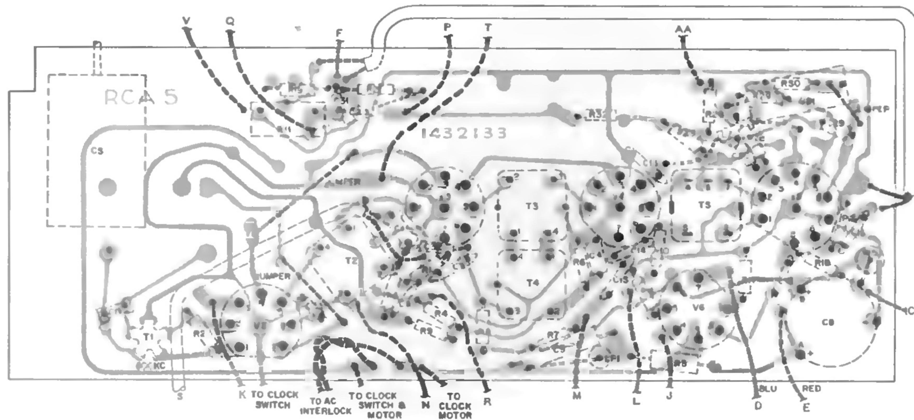
Chassis Layout (Wiring side)
