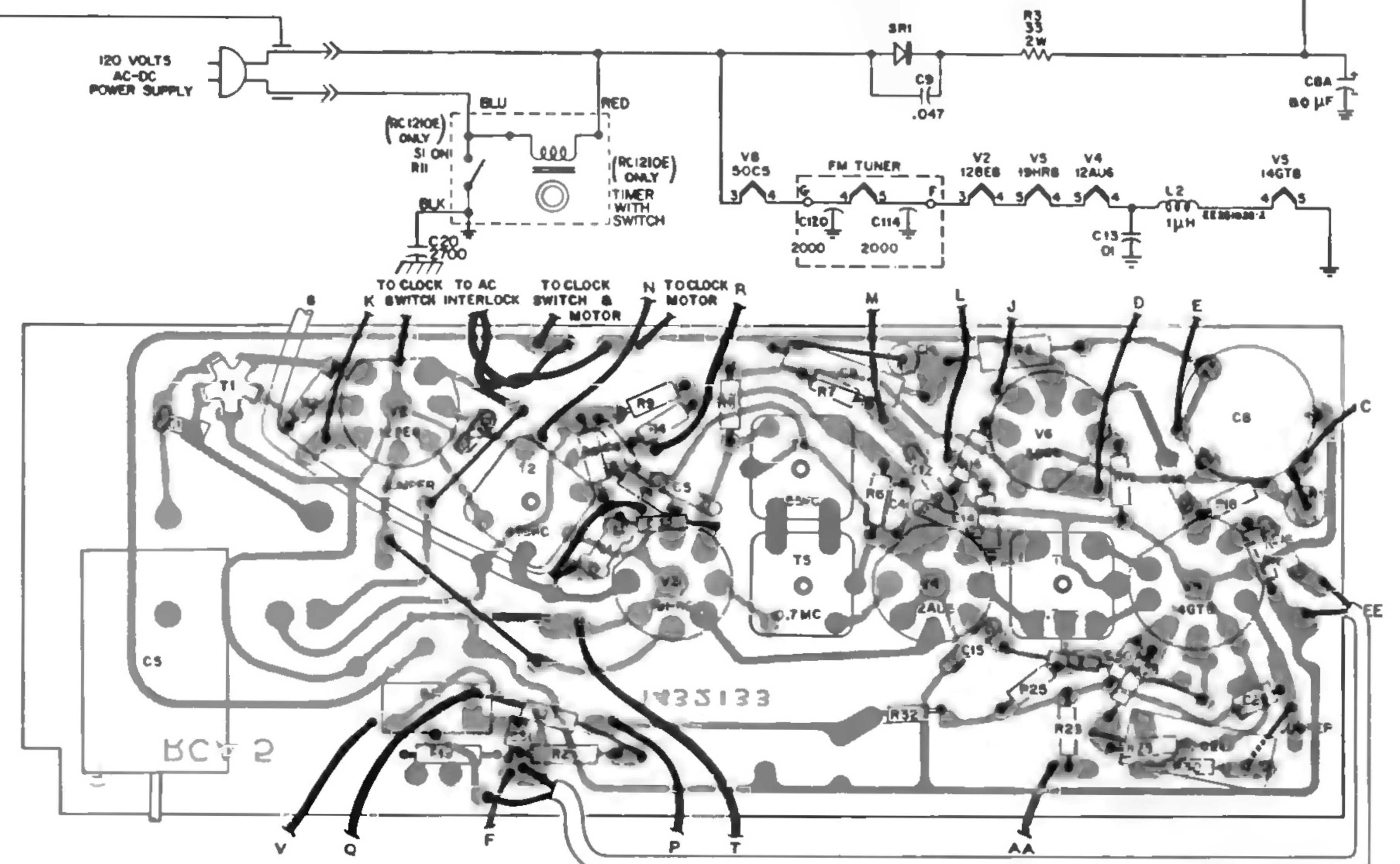
Chassis Layout (Component side)
