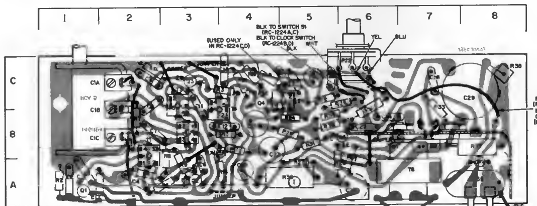
Chassis Layout (Component Side)
