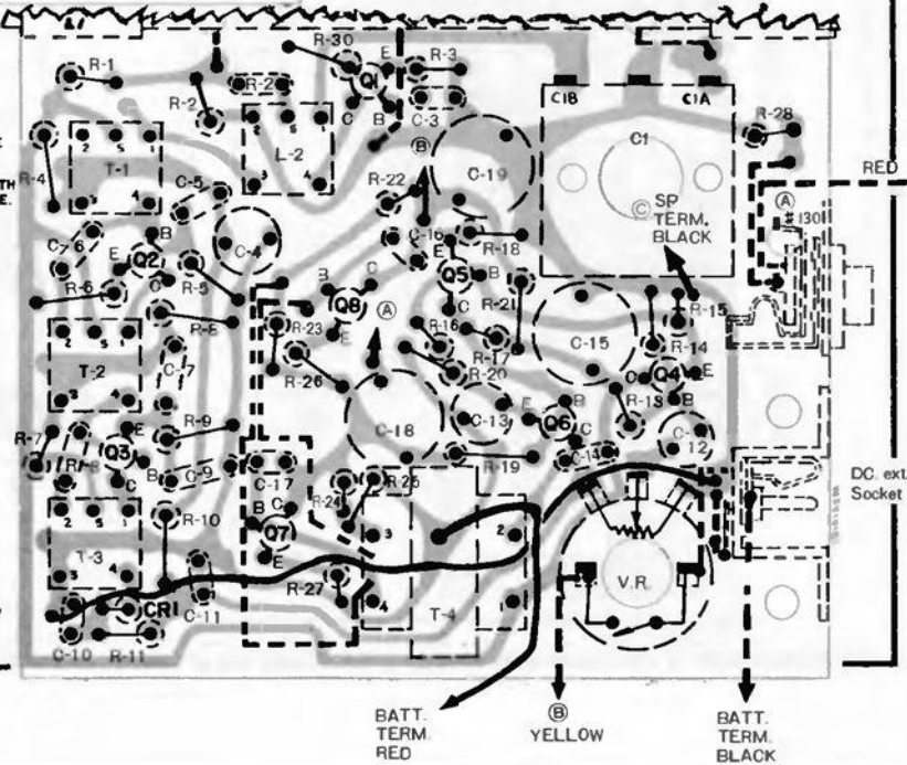
Chassis Layout—Wiring Side →
