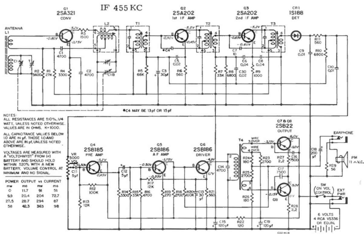
Schematic Diagram
