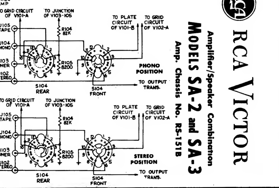
Schematic Diagram of Amplifier RS-151B
