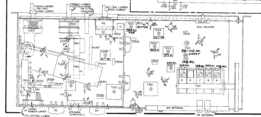
Chassis RC-1227C, E
