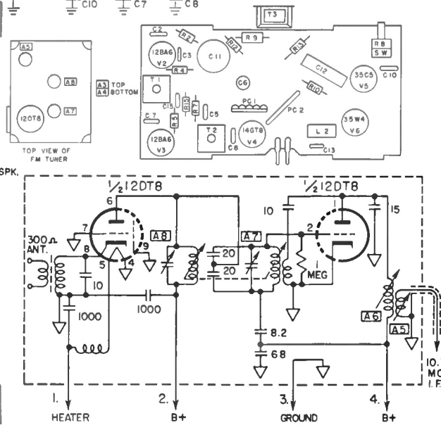
TUNER SCHEMATIC
